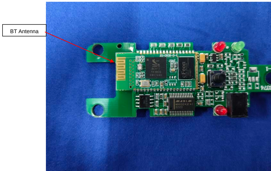
EUT – Bluetooth Module View
