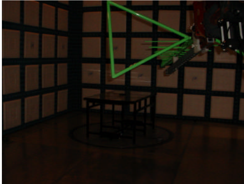
Test Setup for Worst Case Emissions Horizontal Polarity
