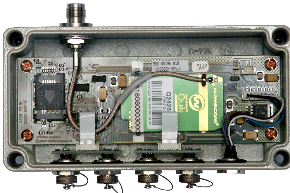
Figure 2.14: A733GSM-USA, Case opened.
