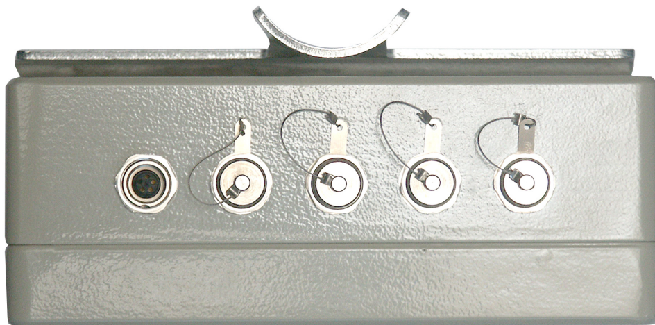
Figure 2.11: A733GSM-USA, Bottom view.
