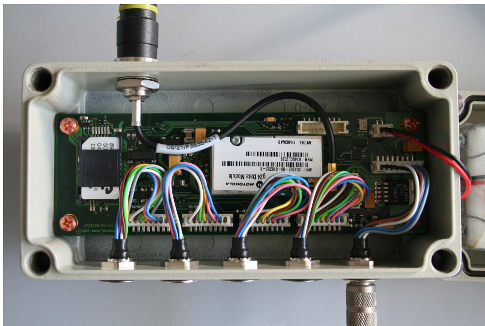
Figure 2.15: A733GSM-GPRS, Case opened.
