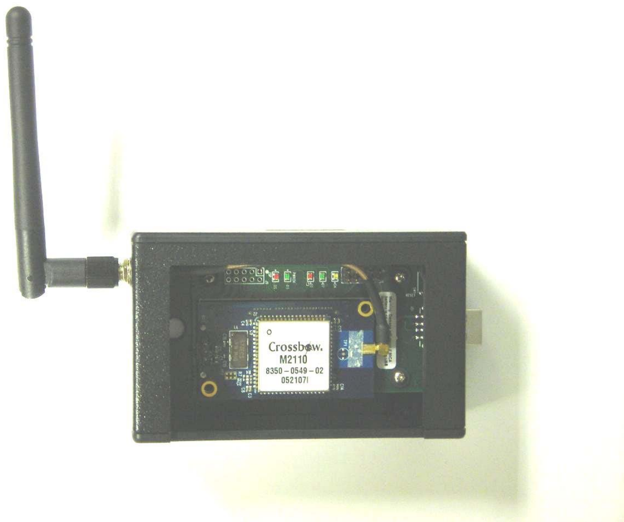
Inside of the Base Station unit
