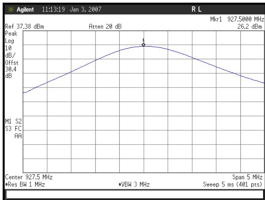
High Ch Peak Power Output
