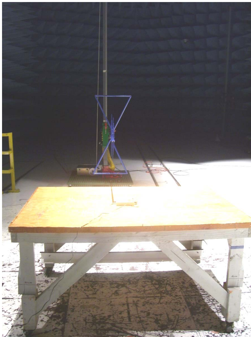
Photograph 4. Radiated Emission Test Setup – Front View
