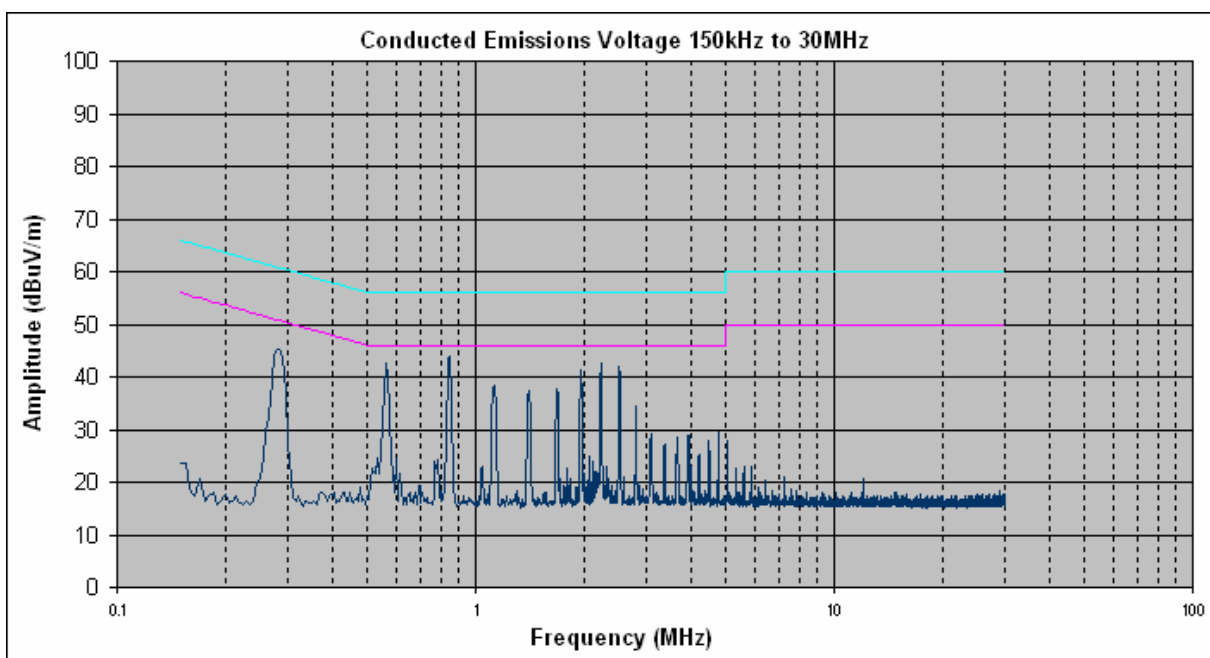
Conducted Emission Limits, Neutral Line Test Results
