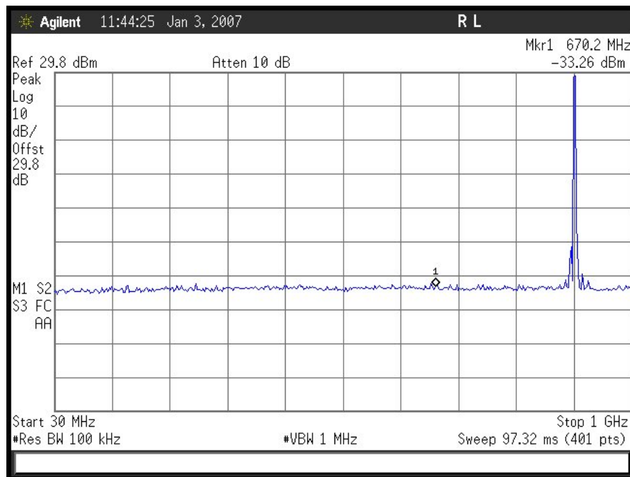
Low Channel Conducted Emissions 30 MHz – 1 GHz
