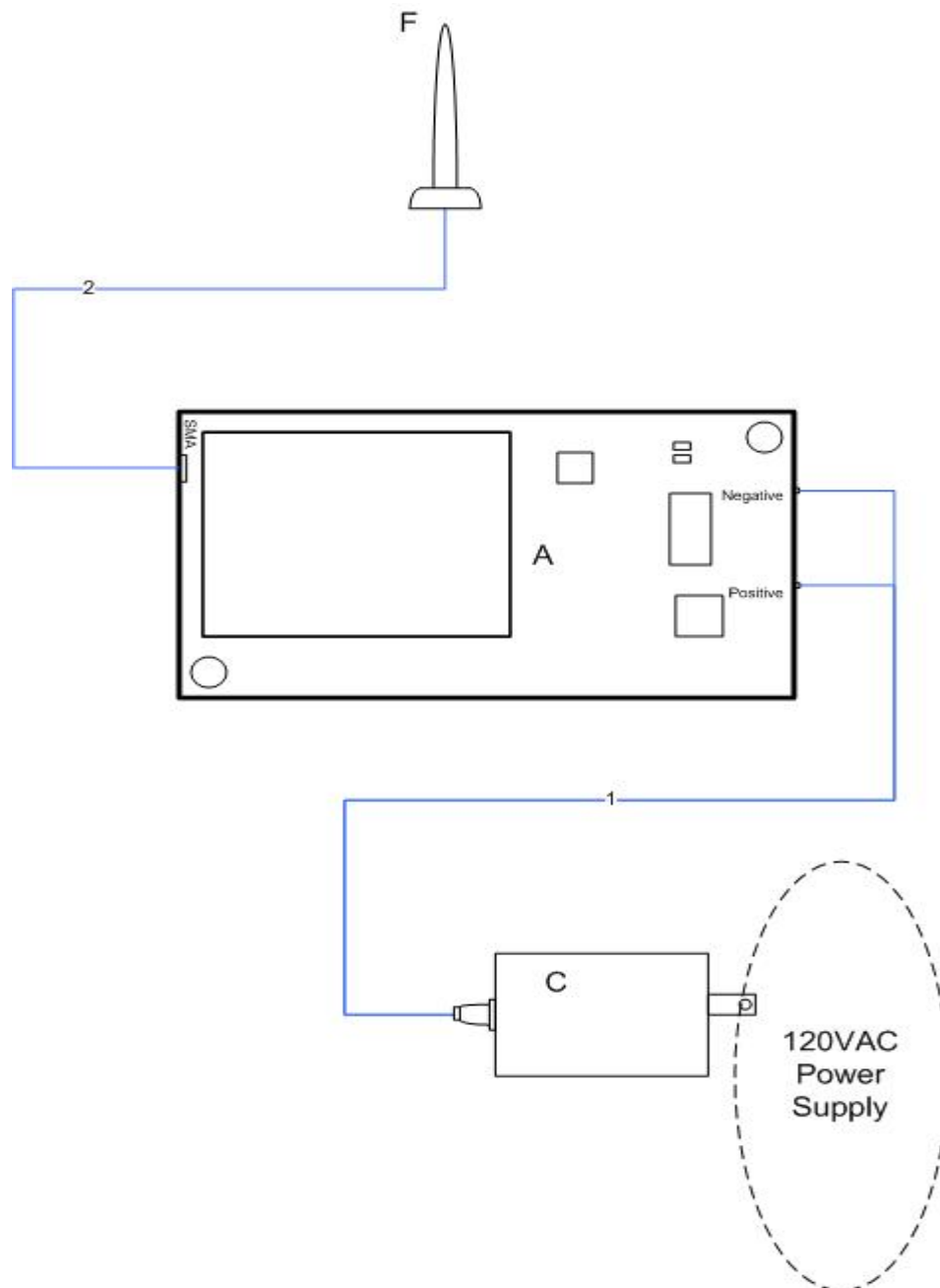
Figure 1. Block Diagram of Test Configuration (Radiated Emissions)
