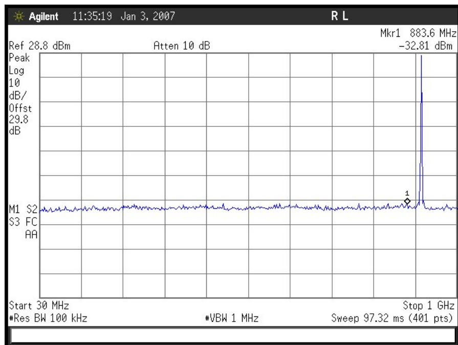
Mid Channel Conducted Emissions 30 MHz – 1 GHz
