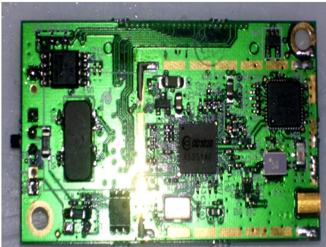
Photograph 1. Crossbow Technology, Inc. MPR1000CB
