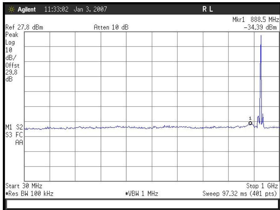
High Channel Conducted Emissions 30 MHz- 1 GHz
