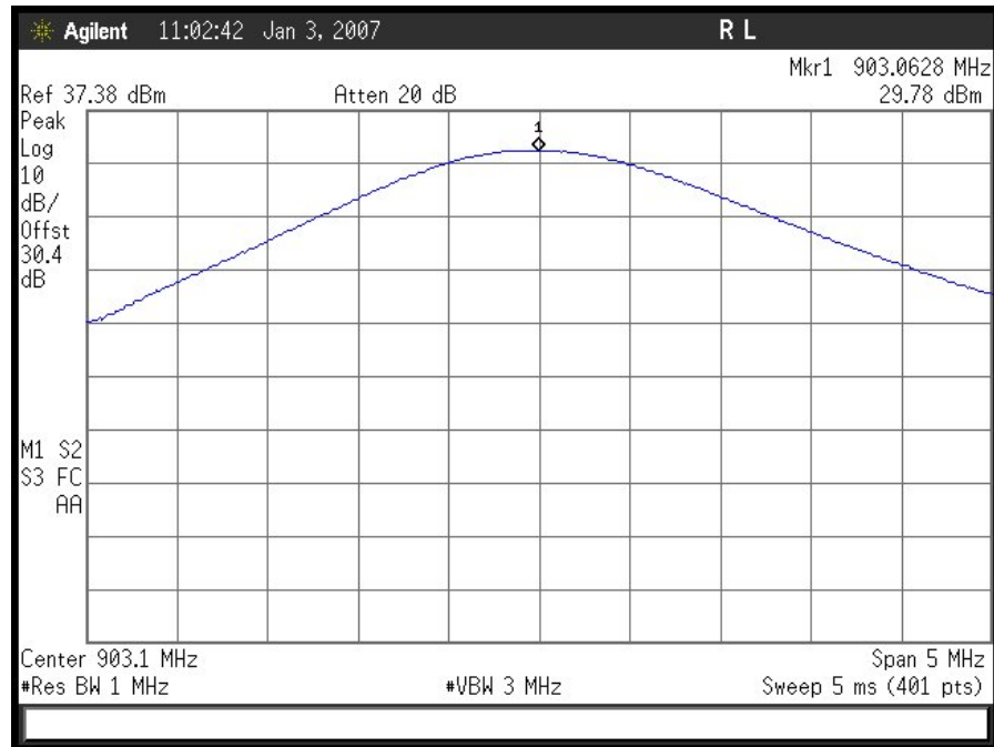
Low Ch Peak Power Output
