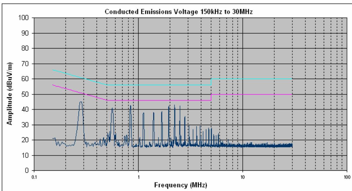
Conducted Emission Limits, Phase Line Test Results
