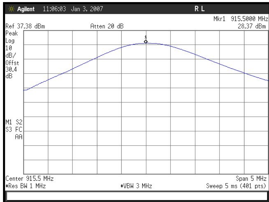
Mid Ch Peak Power Output
