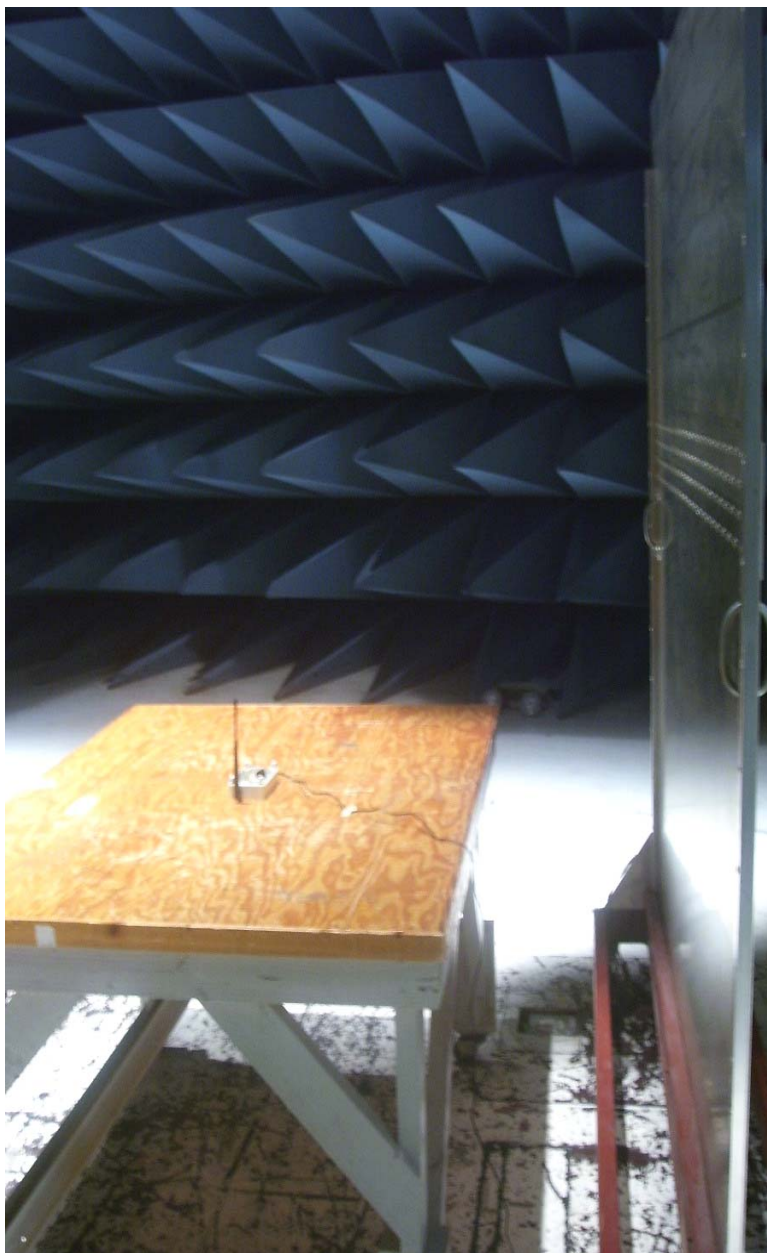
Photograph 7. Conducted Emission Limits Test Setup – Back View
