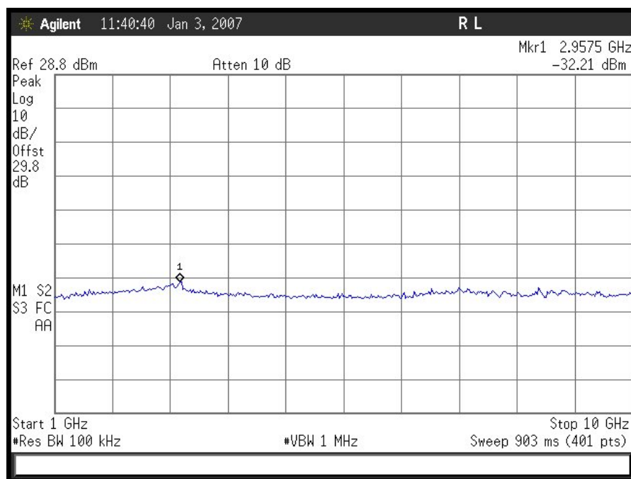
Low Channel Conducted Emissions 1-10 GHz
