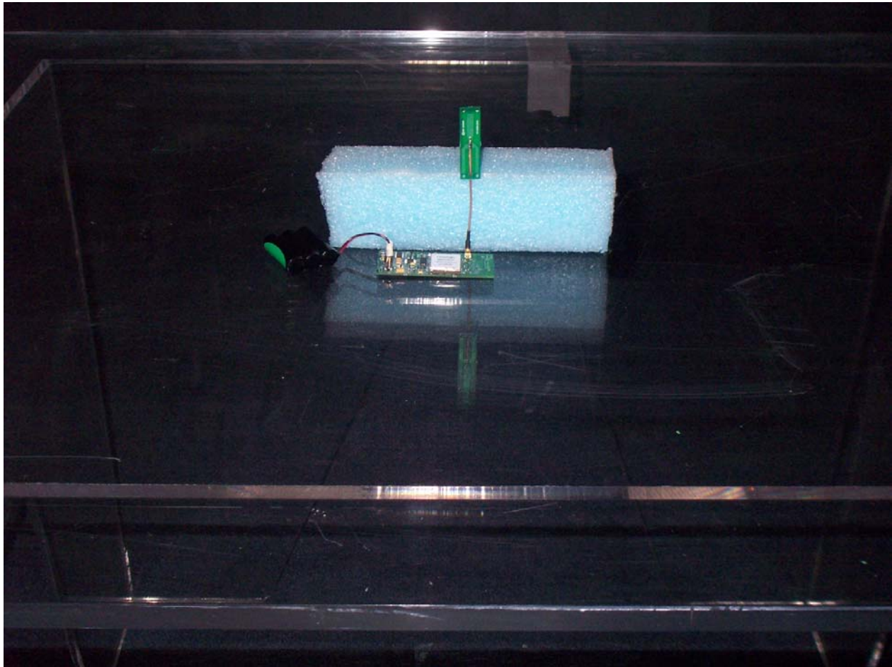
Photograph 1. Radiated Emission Test Setup, 30-1000 MHz
