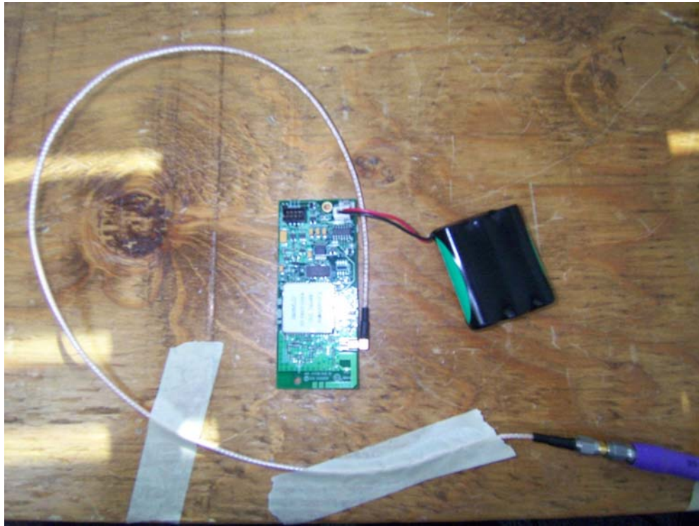
Photograph 3. Spurious Emissions Requirements – Radiated and RF Conducted Test Setup
