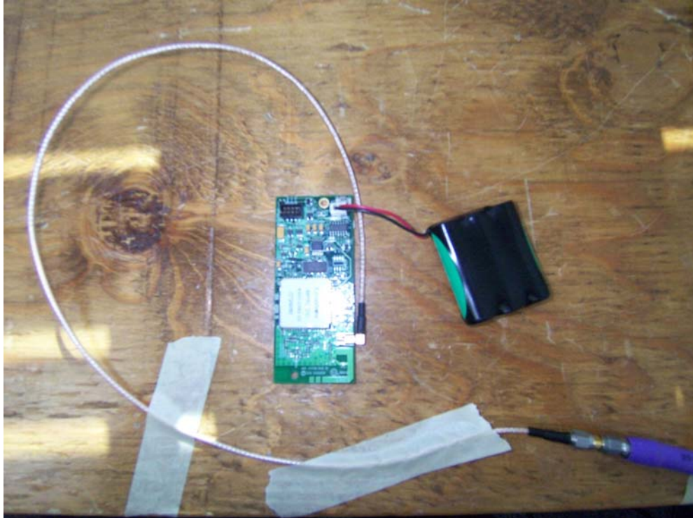
Photograph 5. Spurious Conducted Measurements Test Setup
