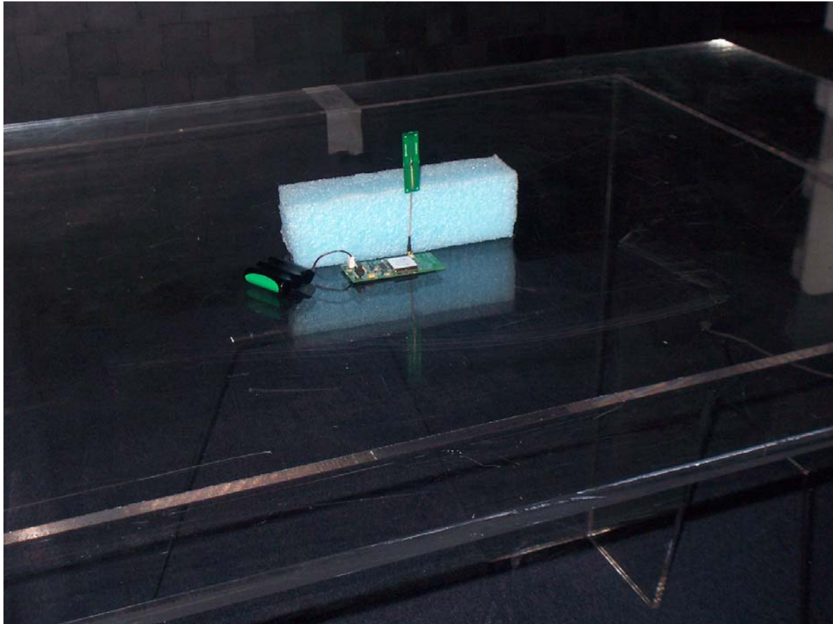
Photograph 4. Spurious Radiated Emissions Measurement Test Setup
