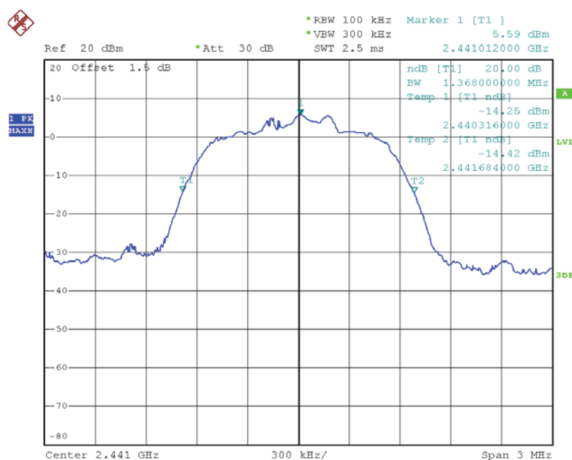
(Plot B: Channel = 2441 @ \pi/4 -DQPSK)
