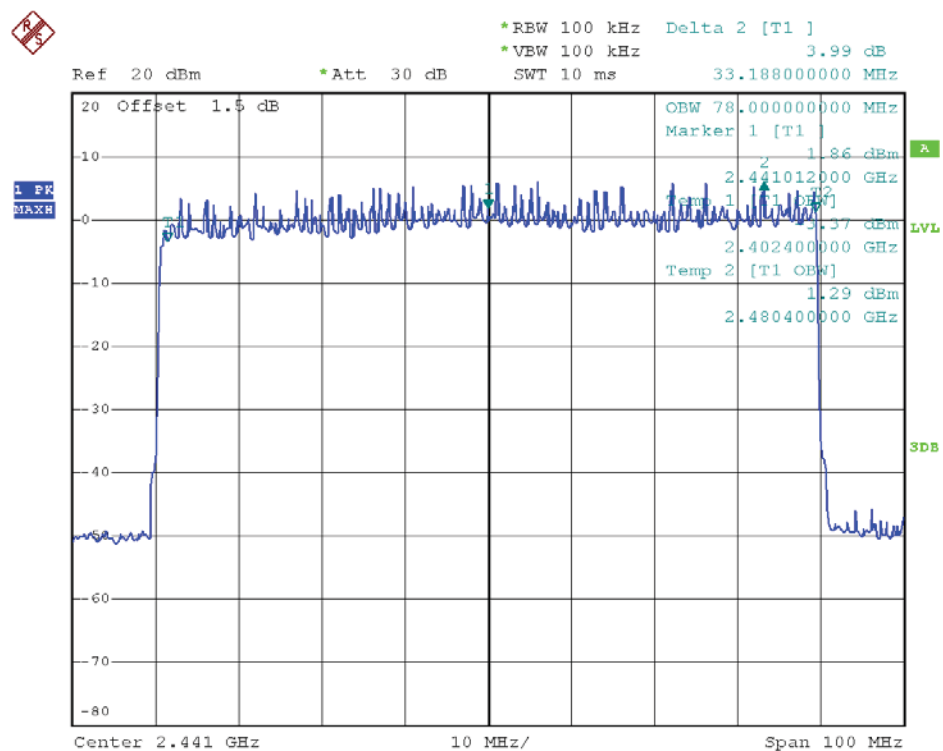
(Plot B:π/4-DQPSK)
