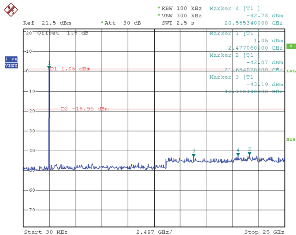
(Plot C: Channel = 78, 30MHz to 25GHz @ 8-DPSK)
