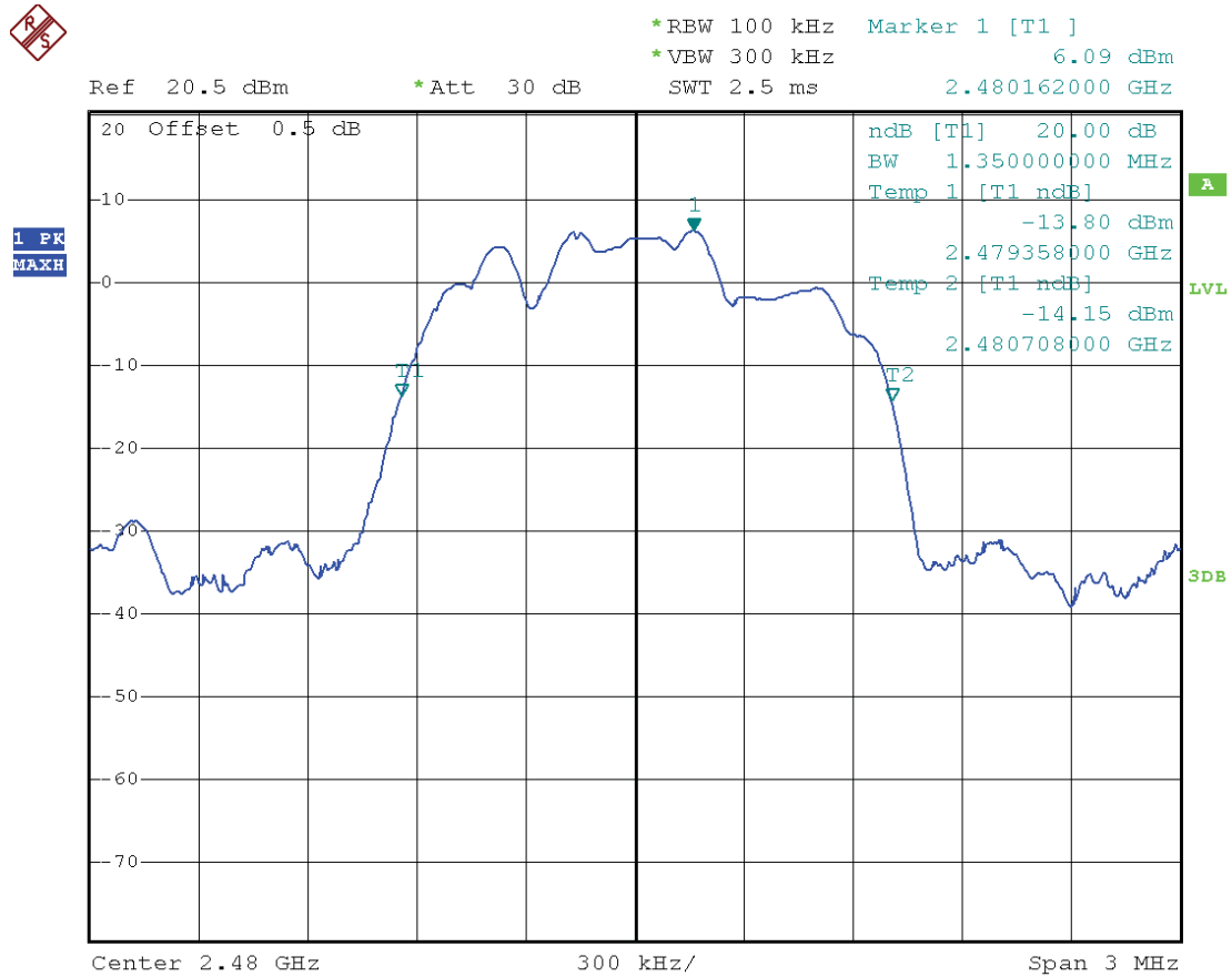
(Plot C: Channel = 2480 @ 8-DPSK)
