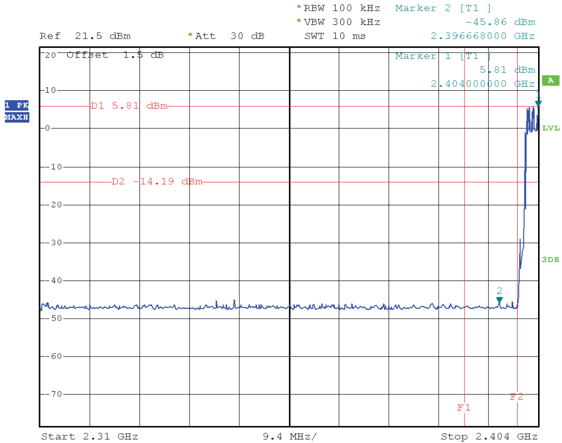
(Plot C1-1: Channel = 0 PEAK)
