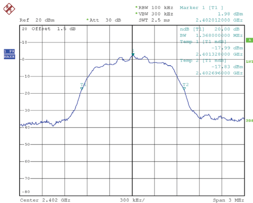
(Plot A: Channel = 2402 @ \pi/4 -DQPSK)
