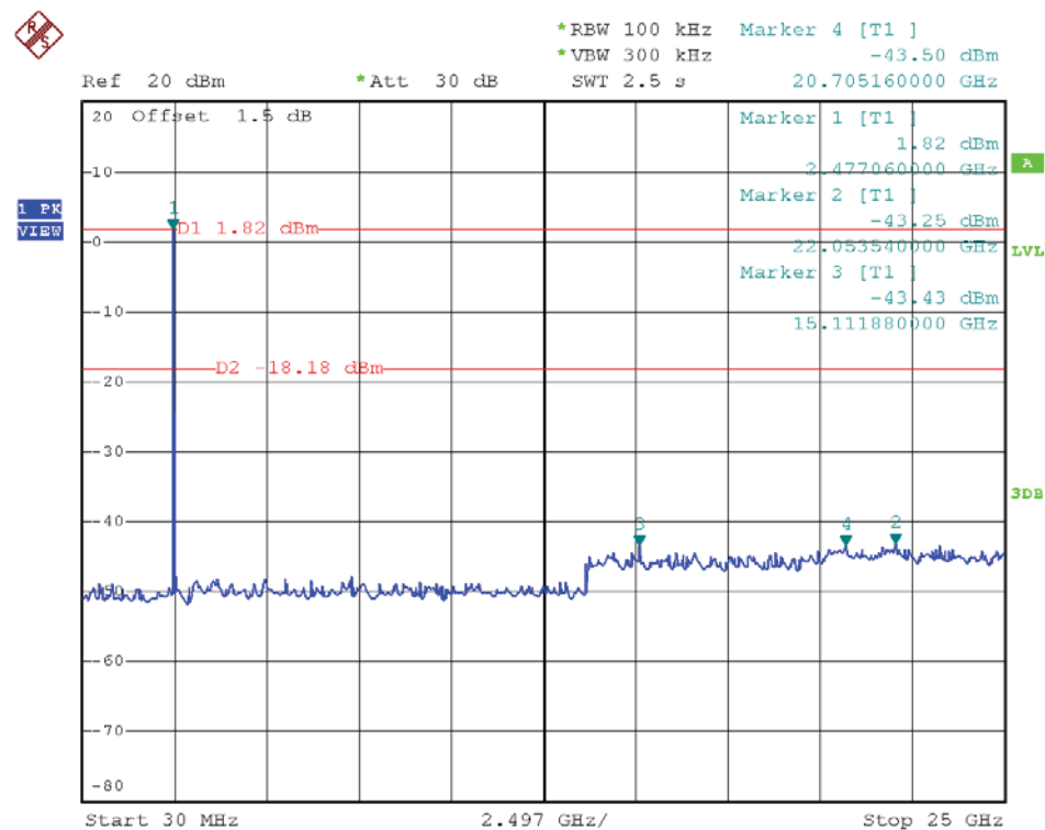
(PlotC: Channel = 78, 30MHz to 25GHz @ \pi/4 -DQPSK)
