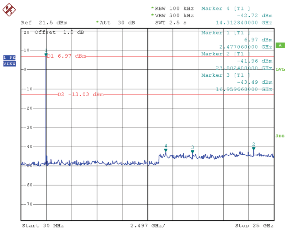
(Plot C: Channel = 78, 30MHz to 25GHz @ GFSK Mode)
