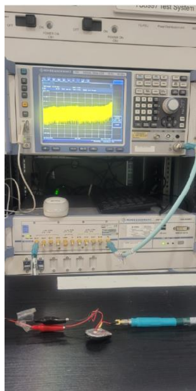
Figure B4. DUT Setup- Conducted
