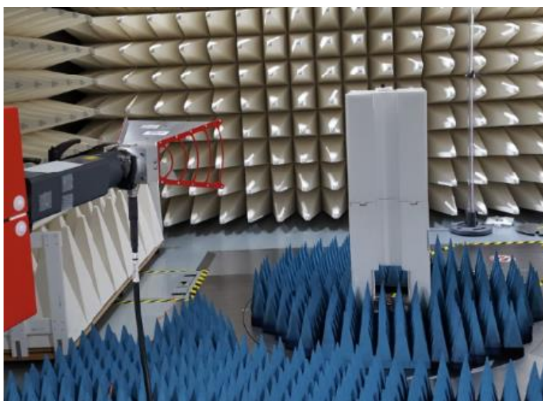
Figure B6. Radiated Test Setup 2
