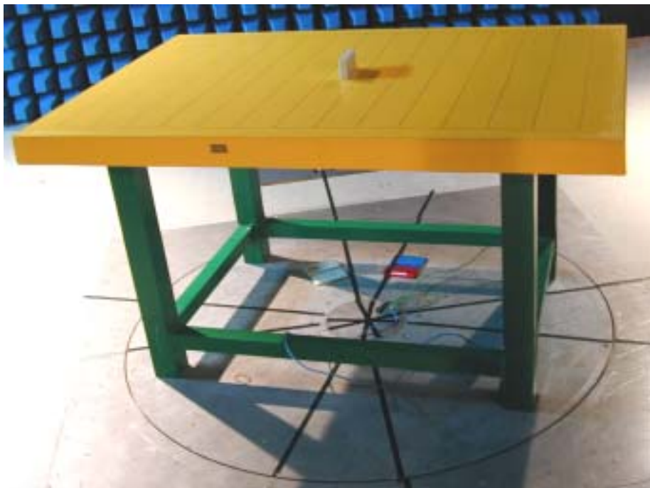
Photo 2: Radiated Emission Test Set-up
