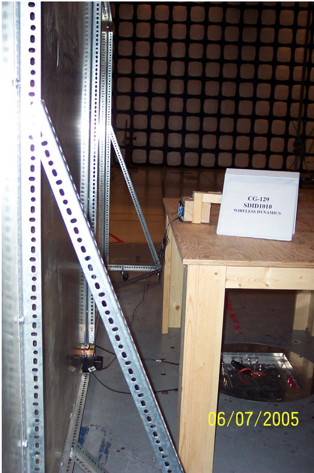
Figure 2 Conducted Emissions Test Photograph
