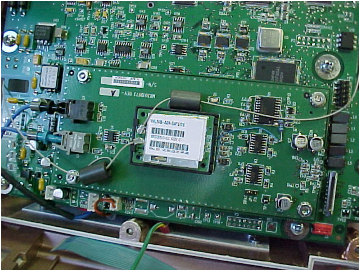
Photo Two – Internal RF PCB mounted on Digital Interface PCB
