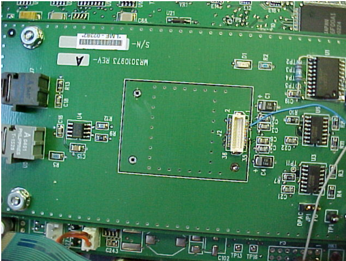
Photo Three – Internal Area RF PCB is mounted on Digital Interface PCB
