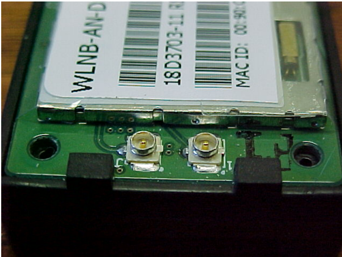
Photo Six – Internal RF Module, prepackaged by DEPAC Airborne Wireless Close Up of Antenna Connections
