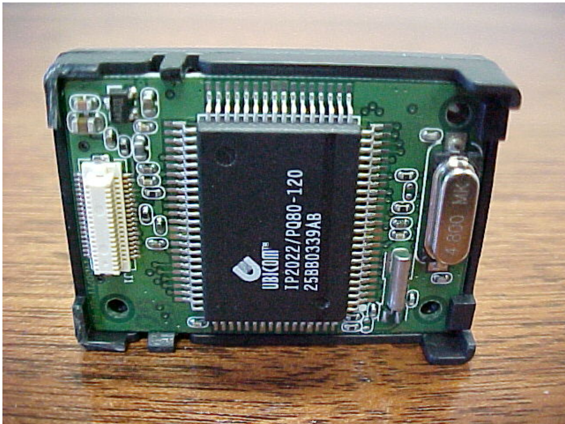
Photo Five – Internal RF Module, prepackaged by DEPAC Airborne Wireless Exposed Side of Pre Packaged Module
