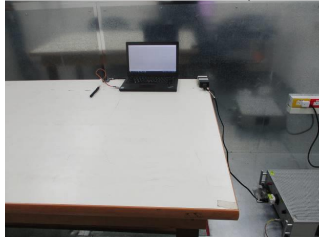
FCC_15_247_WLAN_Conduction_Setup
