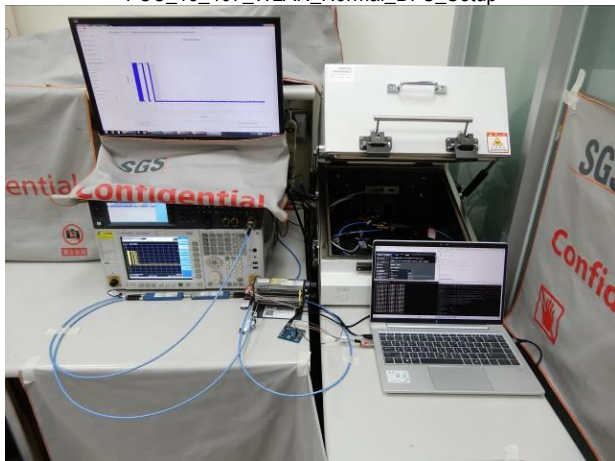
FCC_15_407_WLAN_Normal_DFS_Setup
