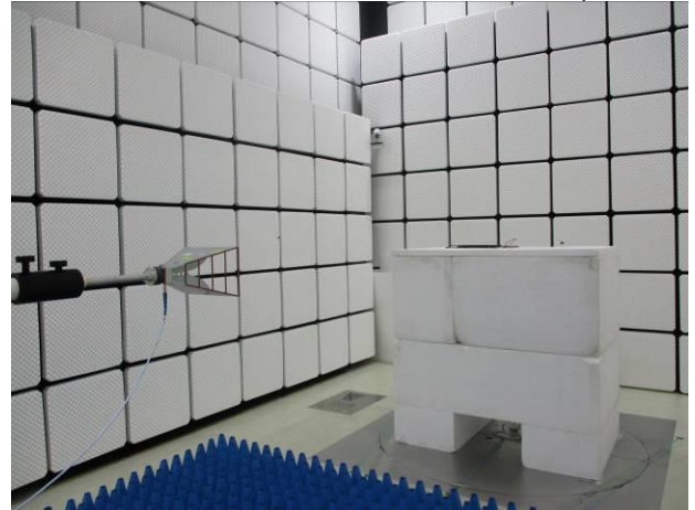
FCC_15_247_WLAN_Radiated_2344655-1_Setup
