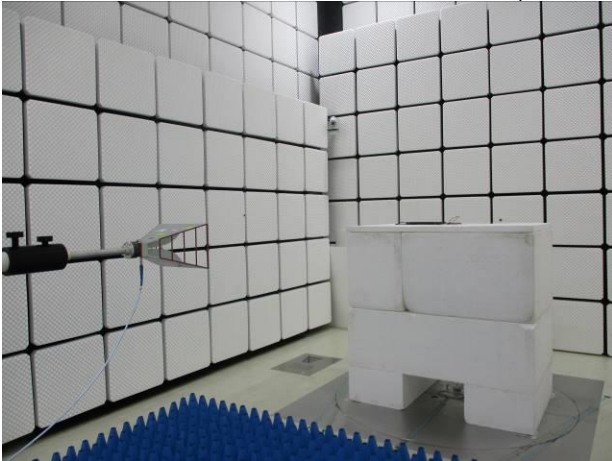
FCC_15_407_WLAN_Radiated_2344655-1_Setup
