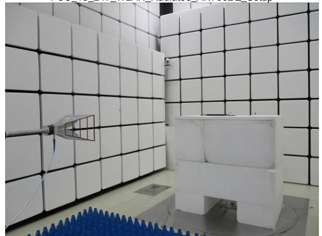
FCC_15_247_WLAN_Radiated_AN7002Q_Setup
