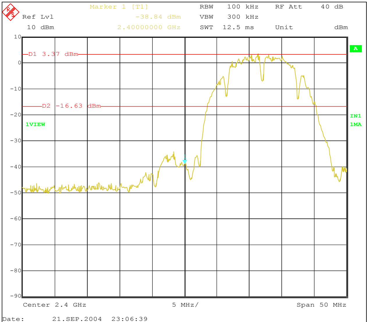
Figure 1: Lower Bandedge
