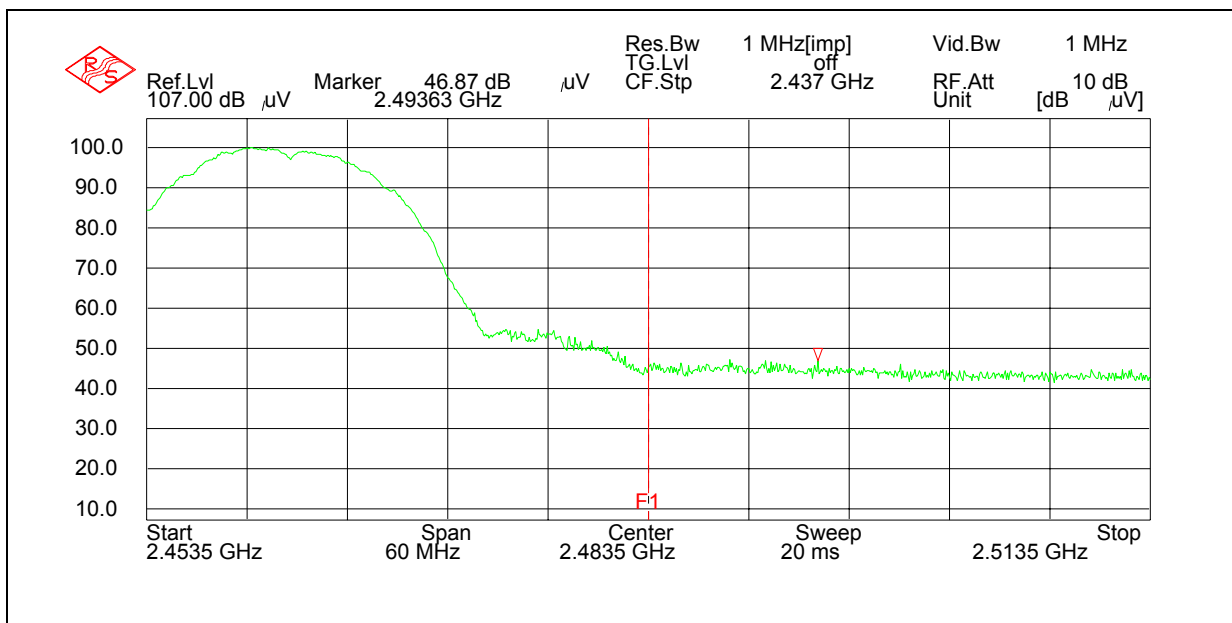
Figure 1: Peak Bandedge Plot
