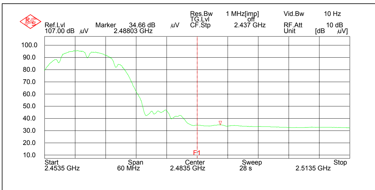
Figure 2: Average Bandedge Plot
