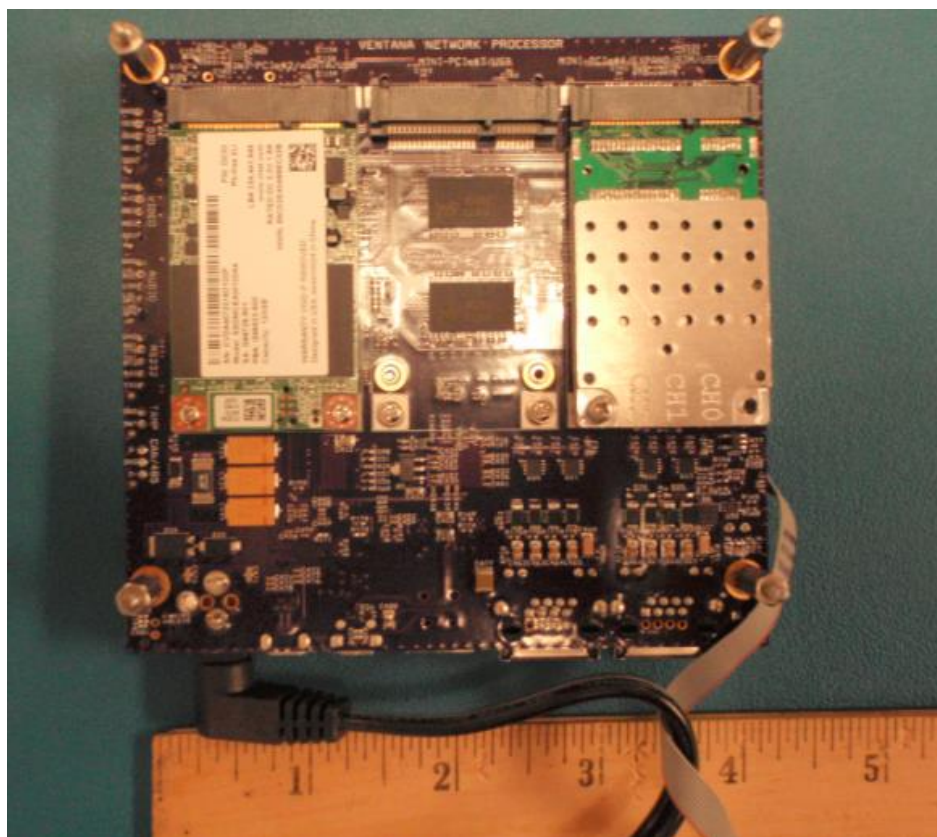
Control Board Top
