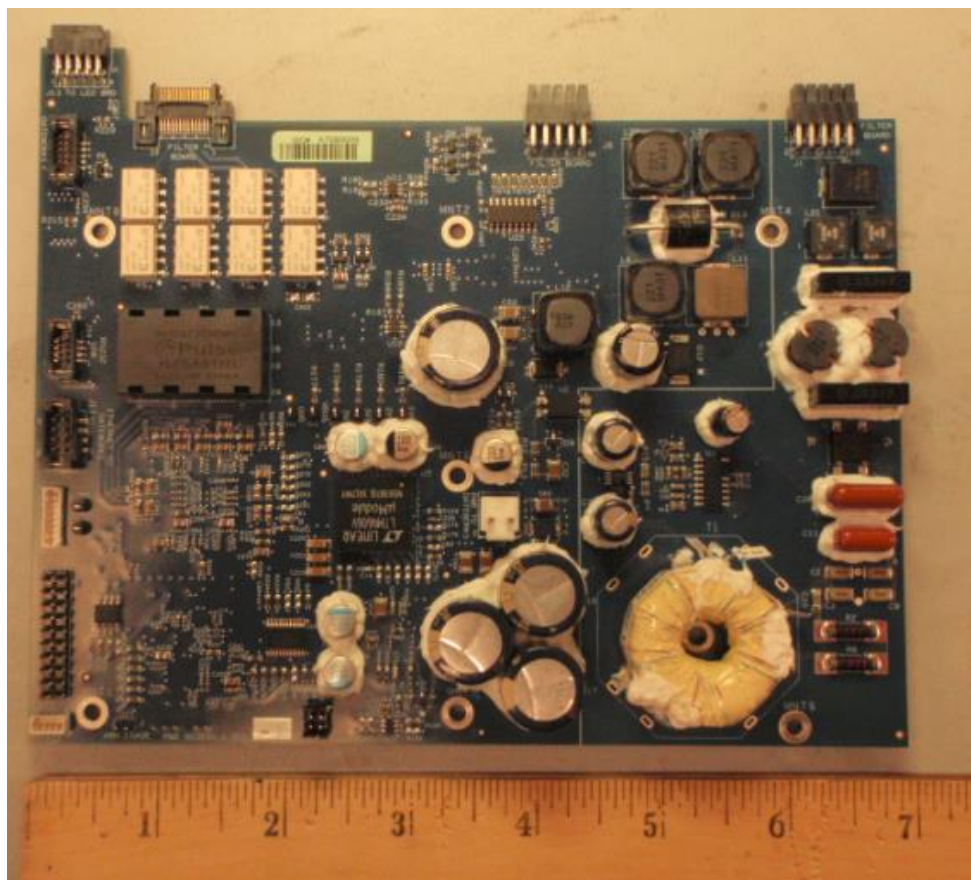
Filter Board Top
