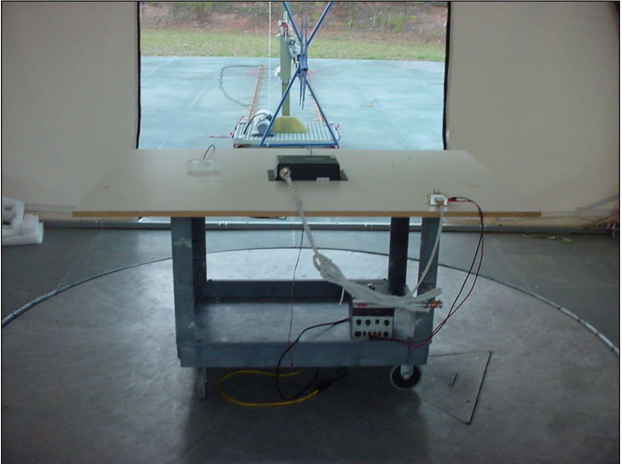
Figure 5: Rear View – WAB
