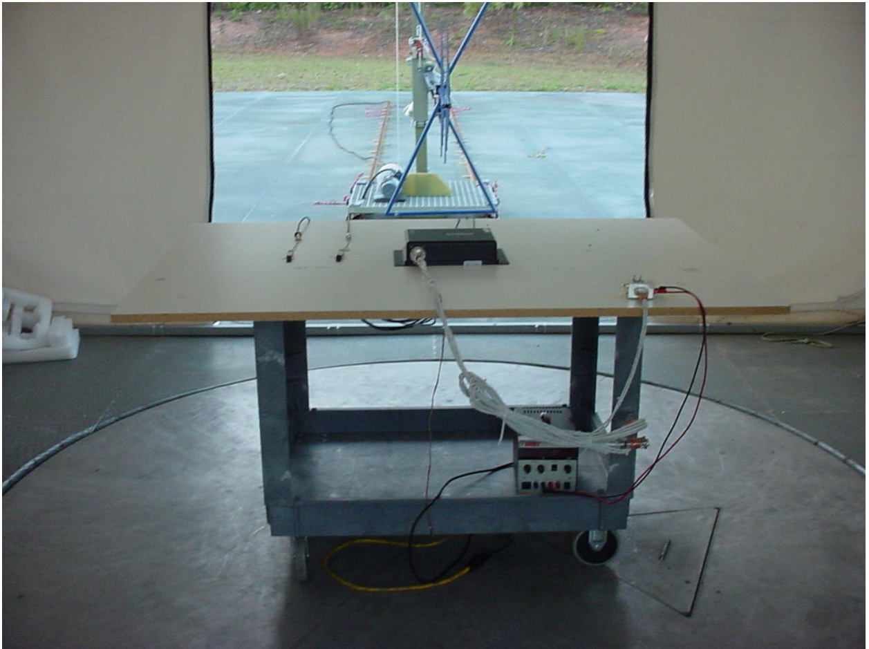
Figure 2: Rear View - CAP
