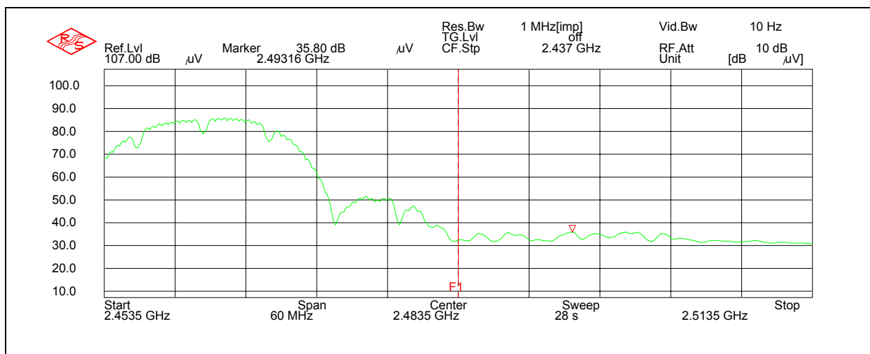
Figure 7.6.3.2-2: Band Edge CAP - Average
