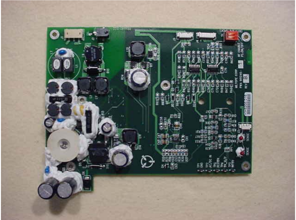
Figure 3: Power Supply PCB – Top View
