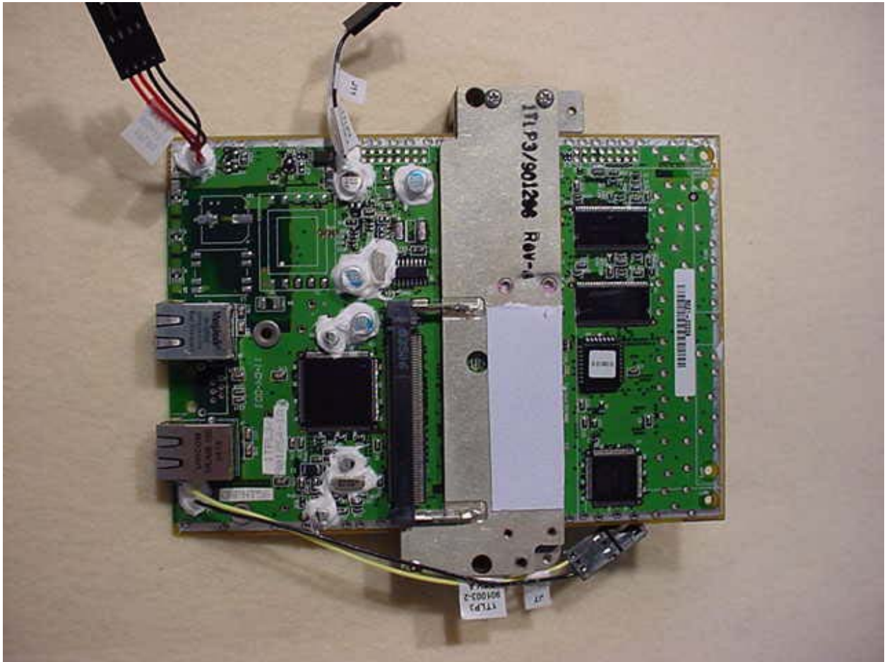
Figure 3: RF PCB – Bottom View
