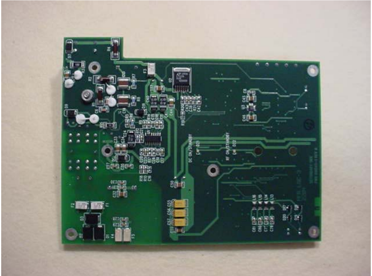
Figure 4: Power Supply PCB – Bottom View
