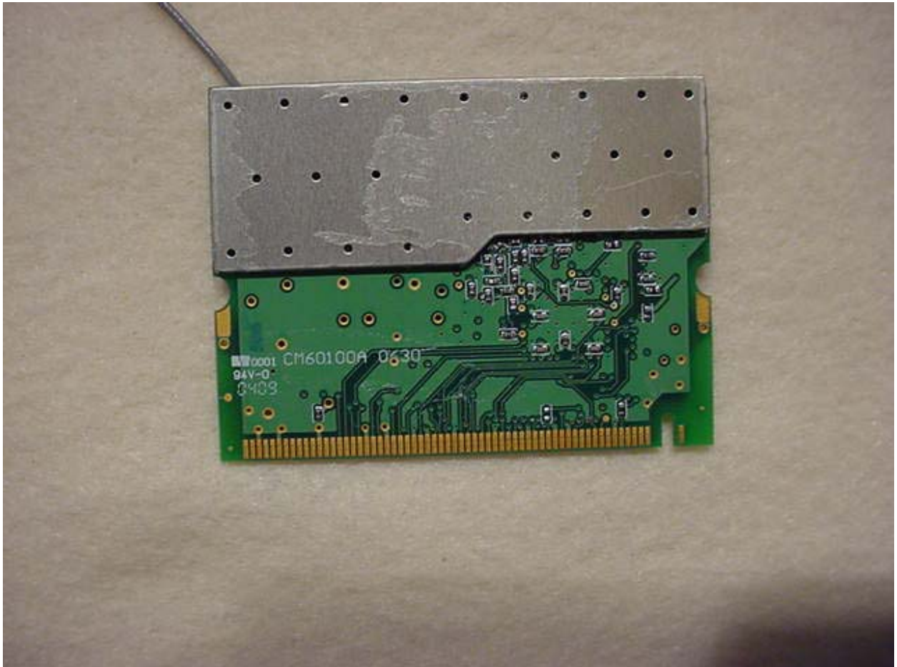
Figure 5: Mini-PCI 802.11 a/b/g Radio Card – Top View
