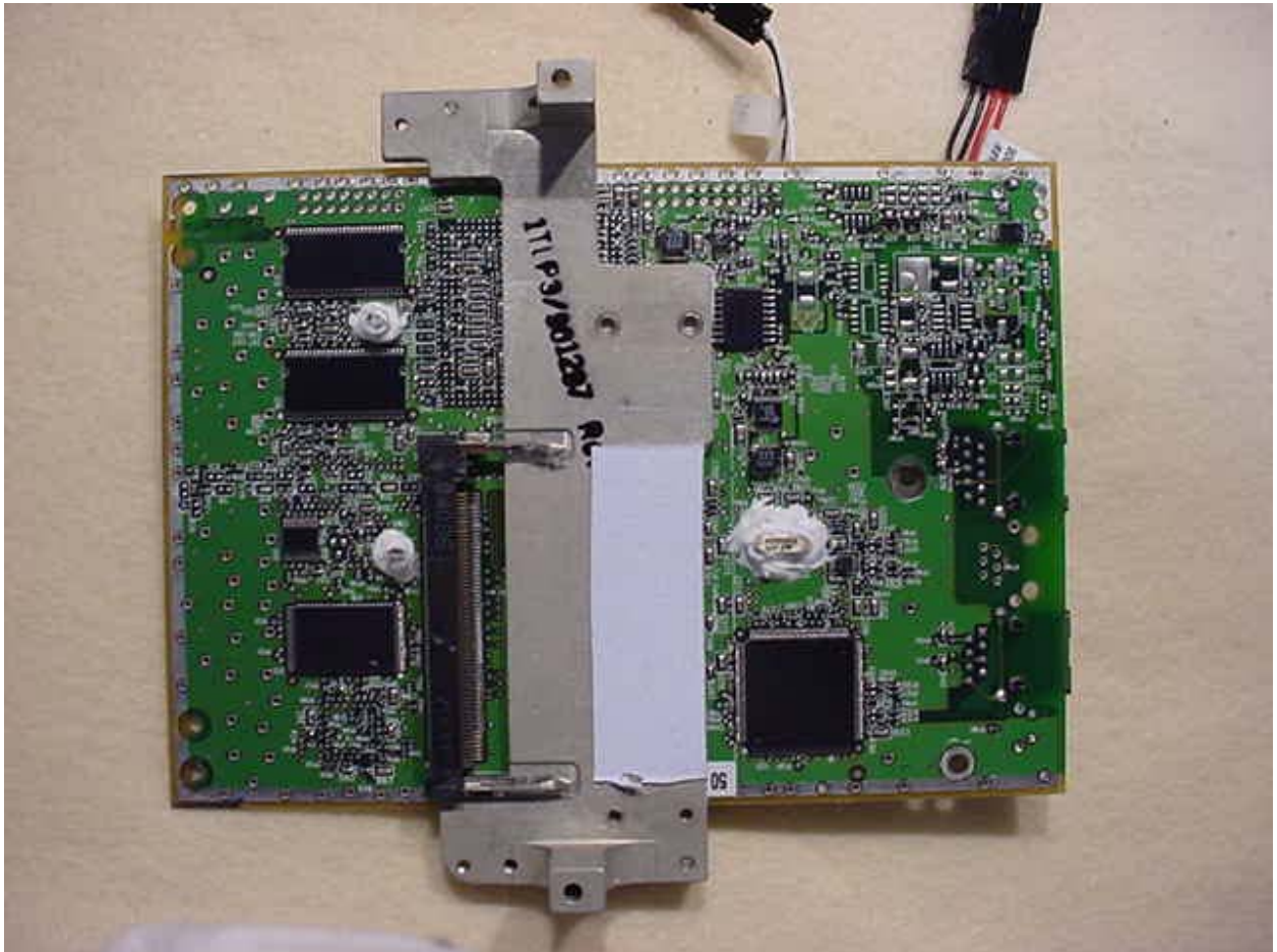
Figure 2: RF PCB – Top View
