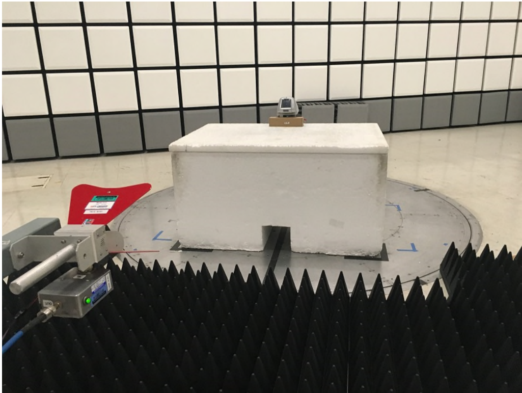
Radiated Emissions Above 1 GHz Front (Unintentional)
