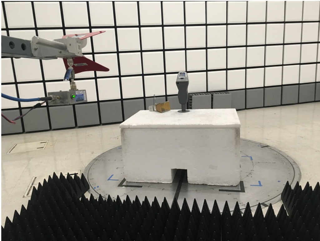
NU Radiated Emissions Above 1GHz Front
