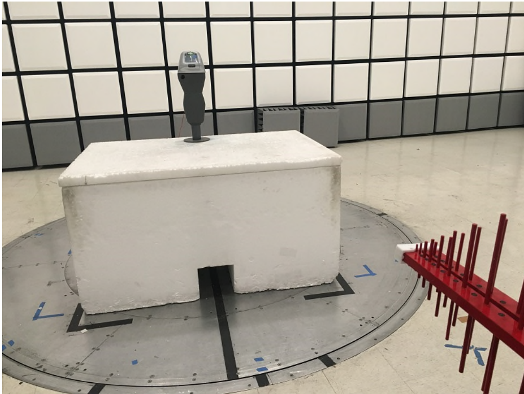
Radiated Emissions 30 MHz to 1 GHz Front
