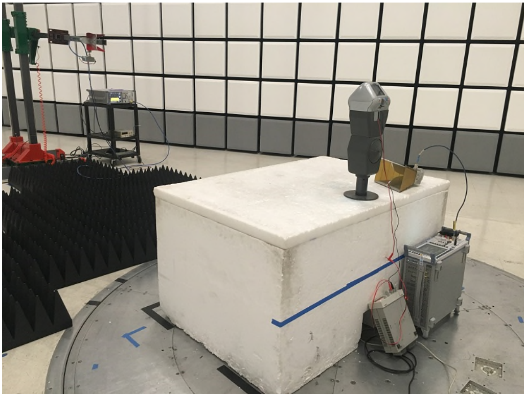
NU Radiated Emissions Above 1GHz Rear
