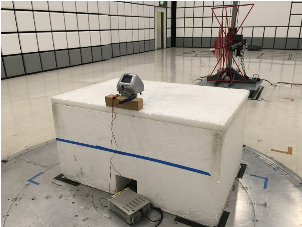
Radiated Emissions Below 1 GHz Rear (Unintentional)
