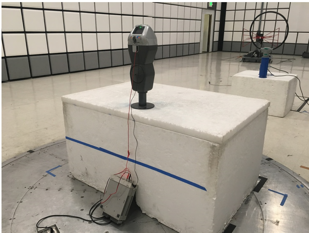
Radiated Emissions Below 30 MHz Rear
