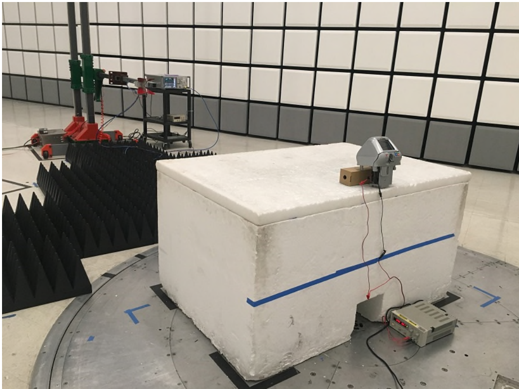
Radiated Emissions Above 1 GHz Rear (Unintentional)
