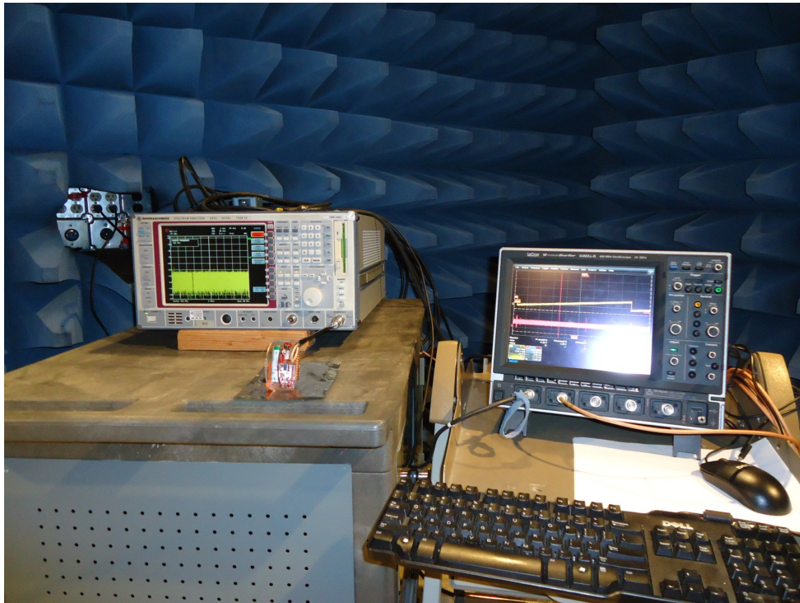
Momentary signals test, 15.231(e )
