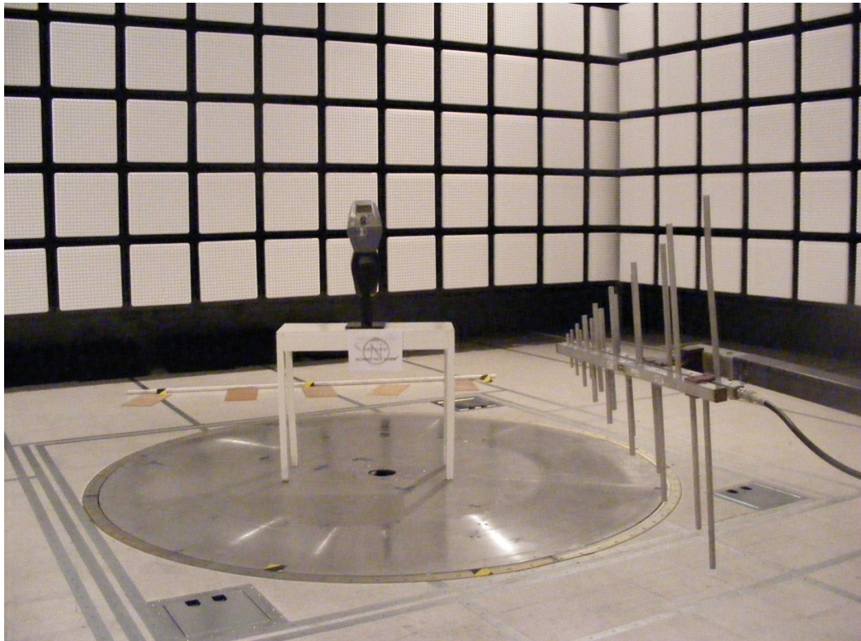
Momentary signals test, 15.231(e )
