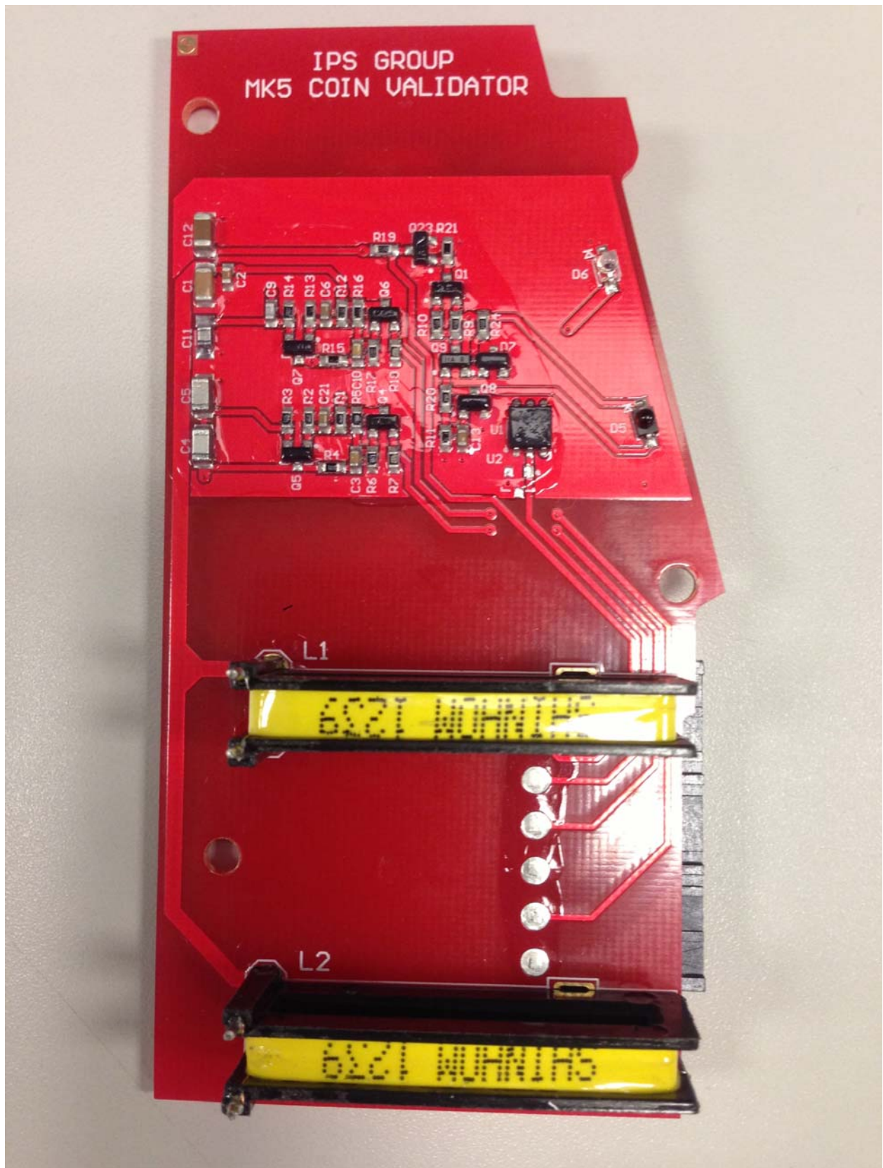
Coin validator card
