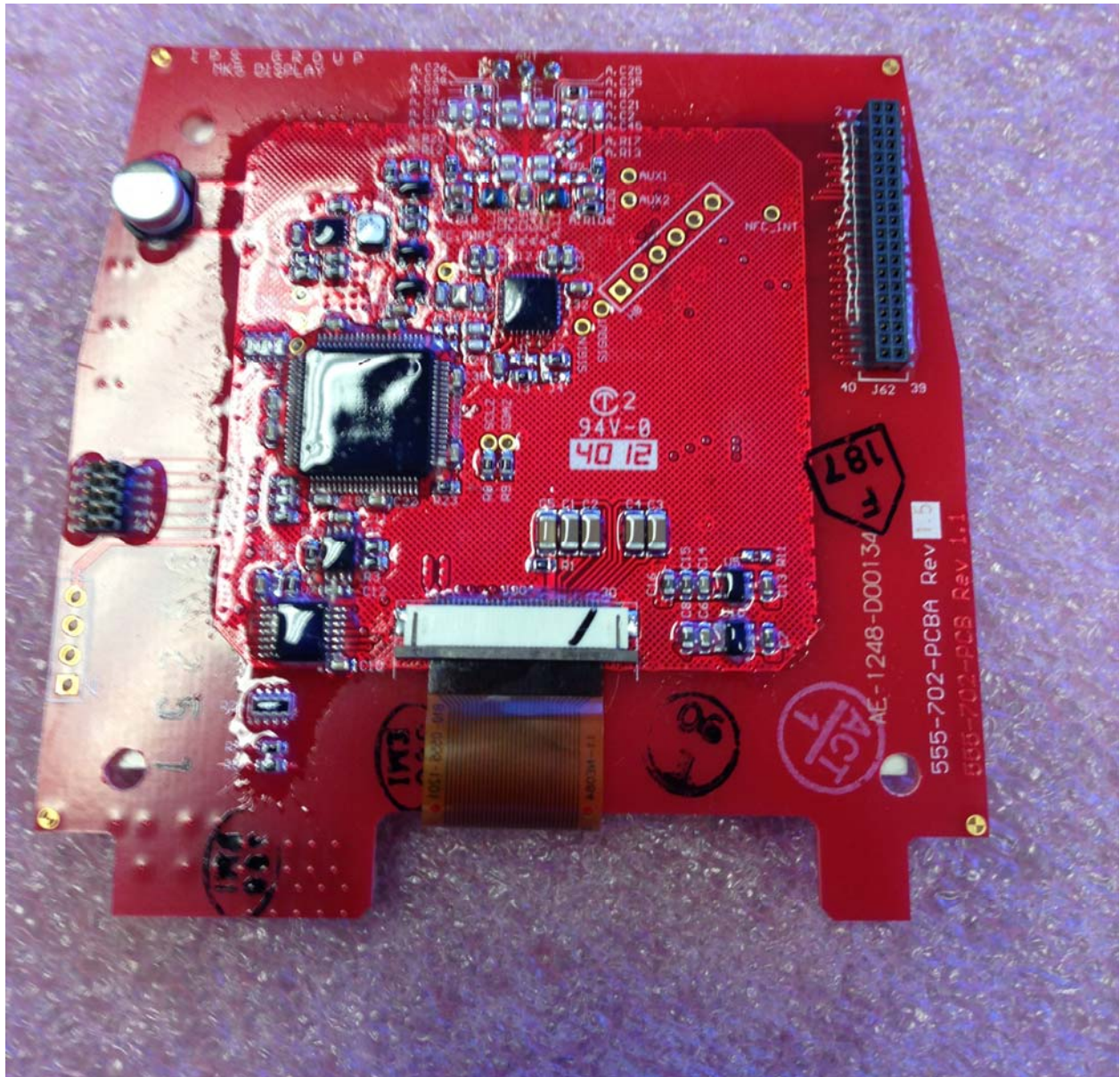
Display board
