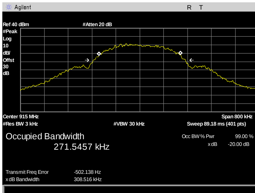
Figure 9: 20dB Bandwidth - 250kbps - mid channel
