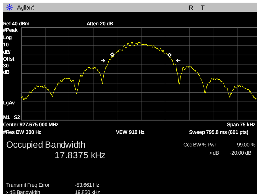
Figure 4: 20dB Bandwidth - 16kbps - high channel
