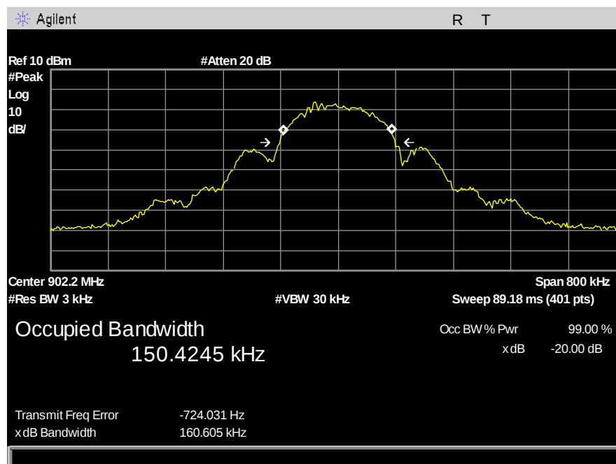
Figure 2: 20dB Bandwidth - 125kbps - low channel
