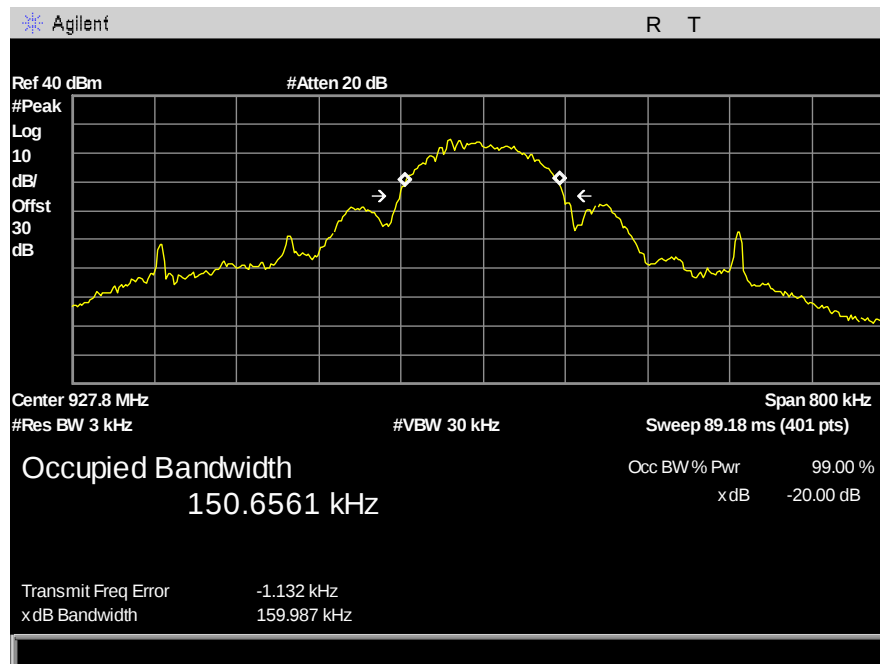
Figure 1: 20dB Bandwidth - 125kbps - high channel
