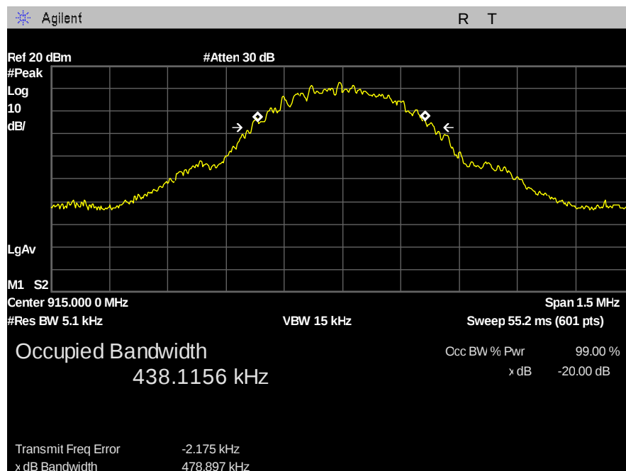
Figure 12: 20dB Bandwidth - 500kbps - mid channel
