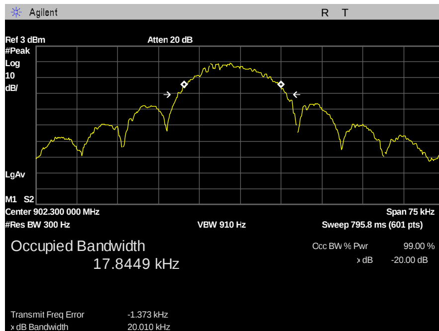
Figure 5: 20dB Bandwidth - 16kbps - low channel
