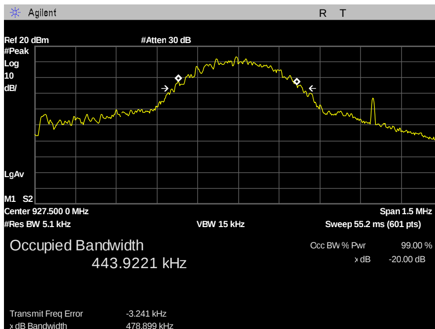
Figure 10: 20dB Bandwidth - 500kbps - high channel
