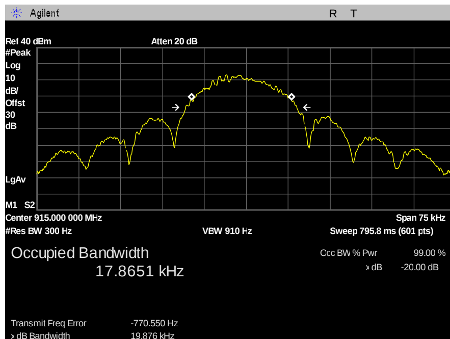
Figure 6: 20dB Bandwidth - 16kbps - mid channel
