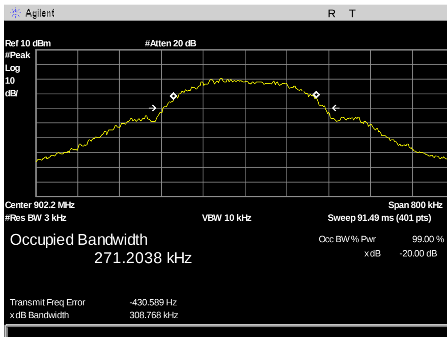
Figure 8: 20dB Bandwidth - 250kbps - low channel
