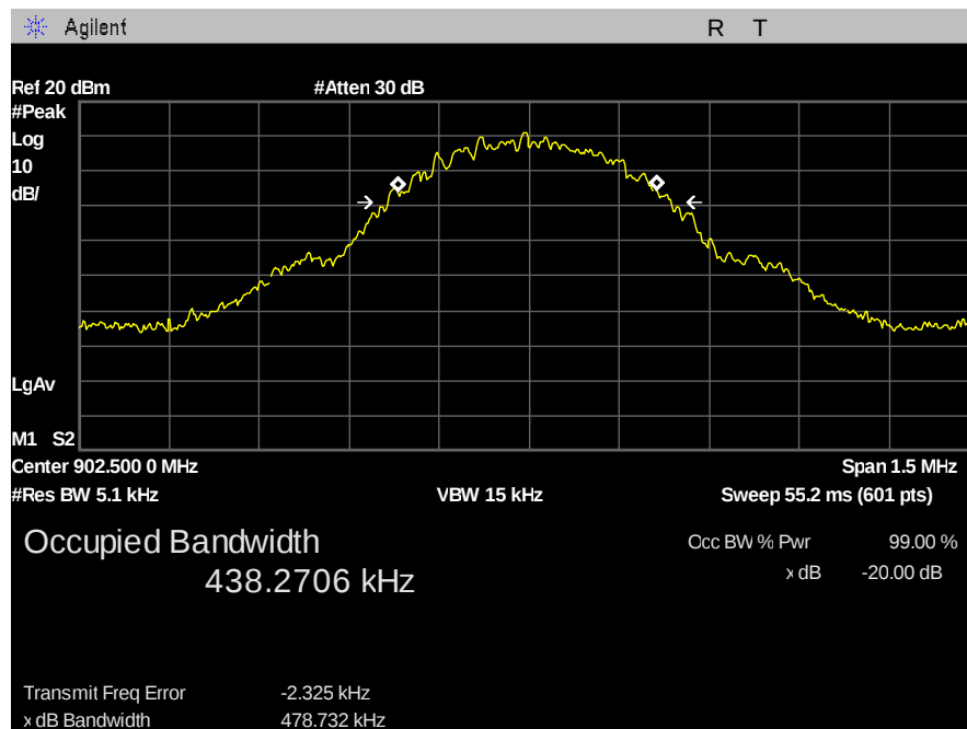
Figure 11: 20dB Bandwidth - 500kbps - low channel
