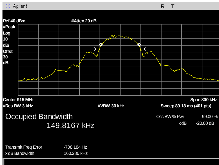
Figure 3: 20dB Bandwidth - 125kbps - mid channel
