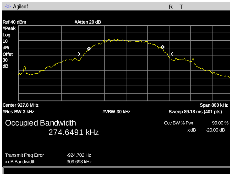
Figure 7: 20dB Bandwidth - 250kbps - high channel
