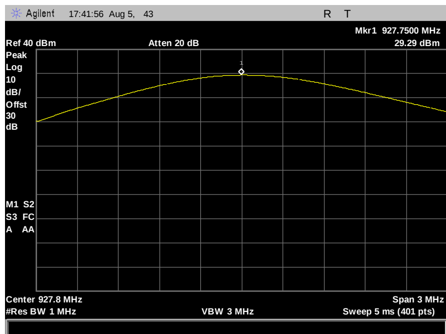
Figure 16: Peak Power - 250kbps - 1dBi - high channel
