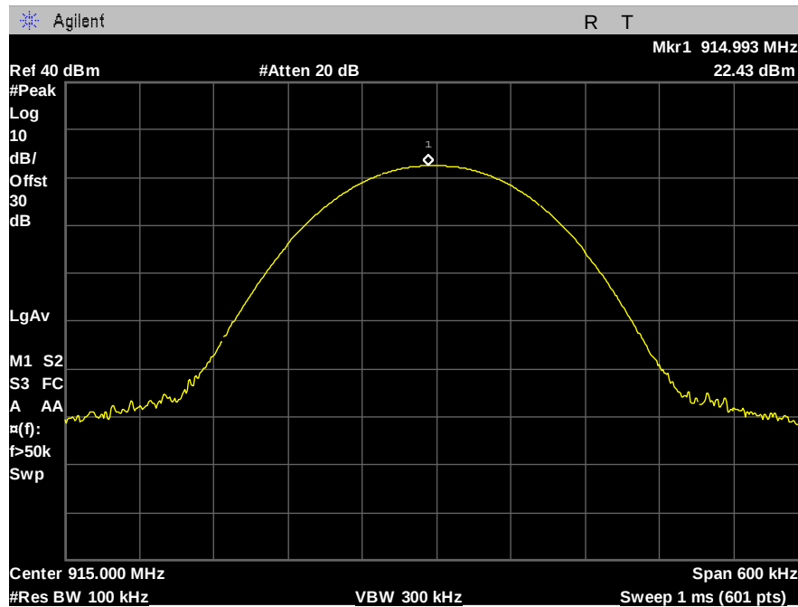
Figure 9: Peak Power - 16kbps - 12dBi - mid channel
