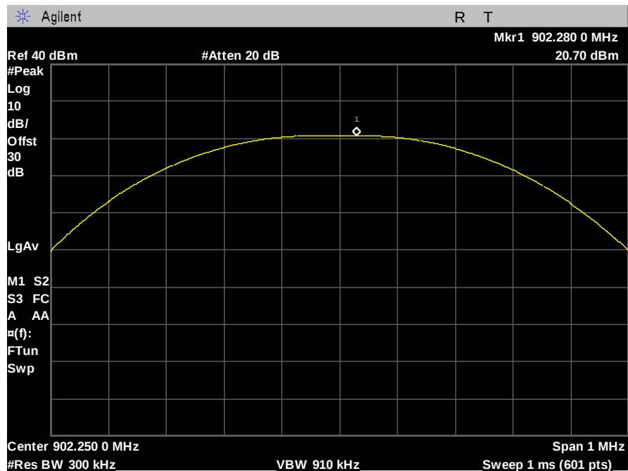
Figure 2: Peak Power - 125kbps - 12dBi - low channel
