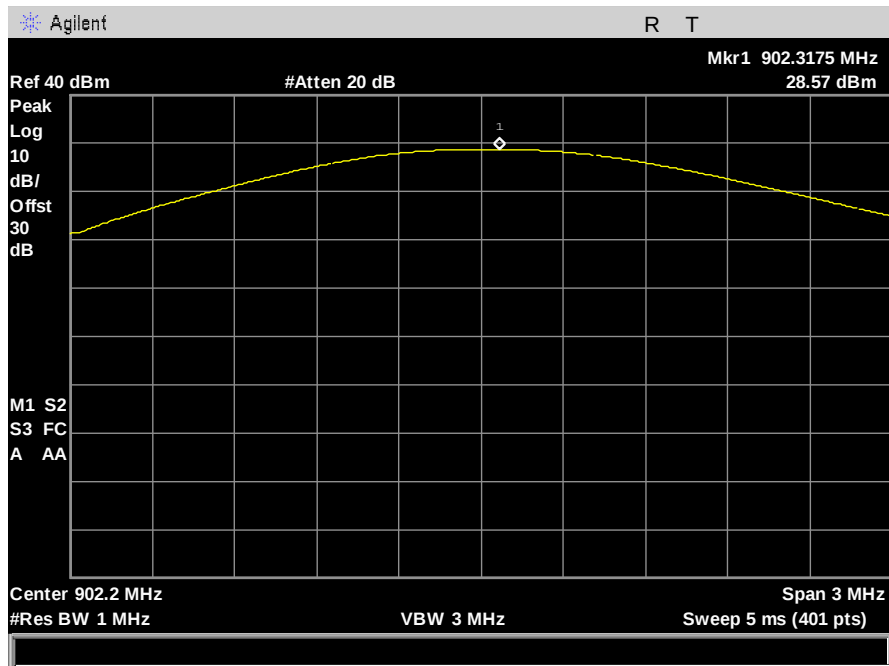
Figure 17: Peak Power - 250kbps - 1dBi - low channel
