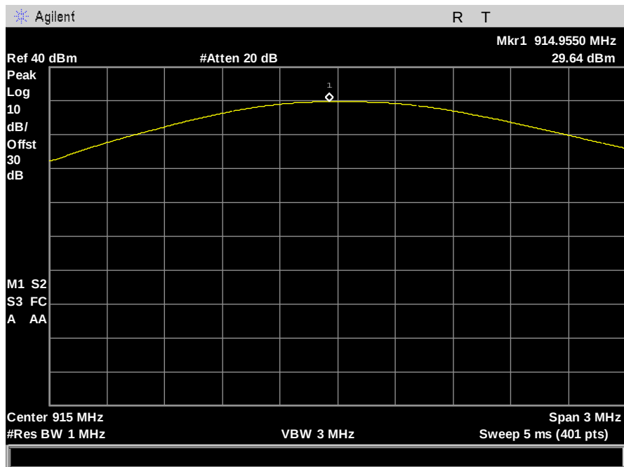
Figure 18: Peak Power - 250kbps - 1dBi - mid channel
