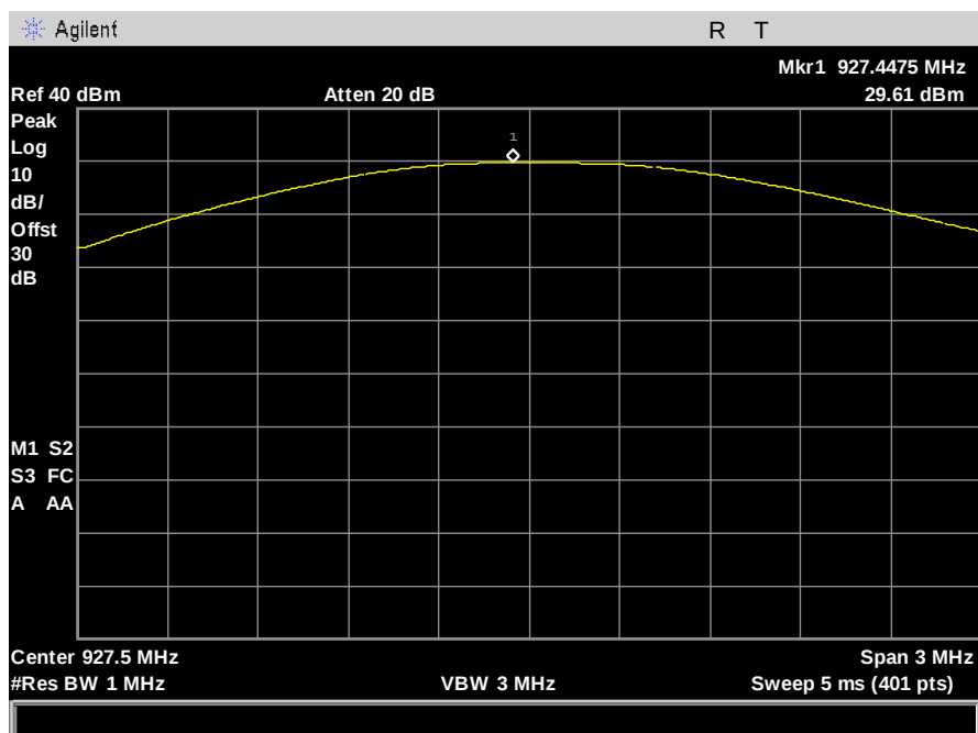
Figure 22: Peak Power - 500kbps - 1dBi - high channel
