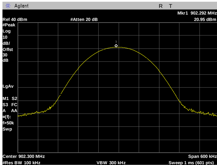
Figure 8: Peak Power - 16kbps - 12dBi - low channel
