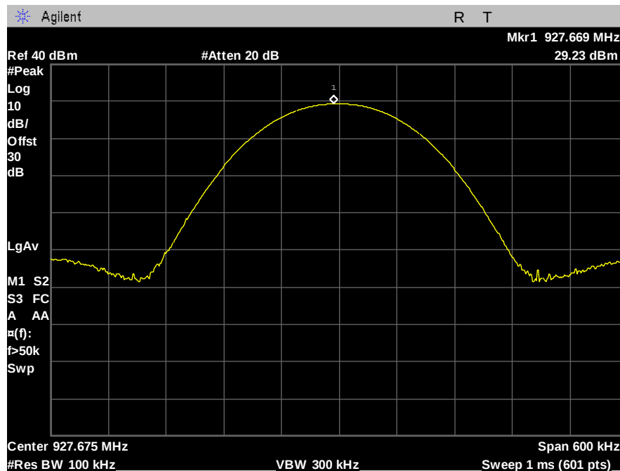
Figure 10: Peak Power - 16kbps - 1dBi - high channel
