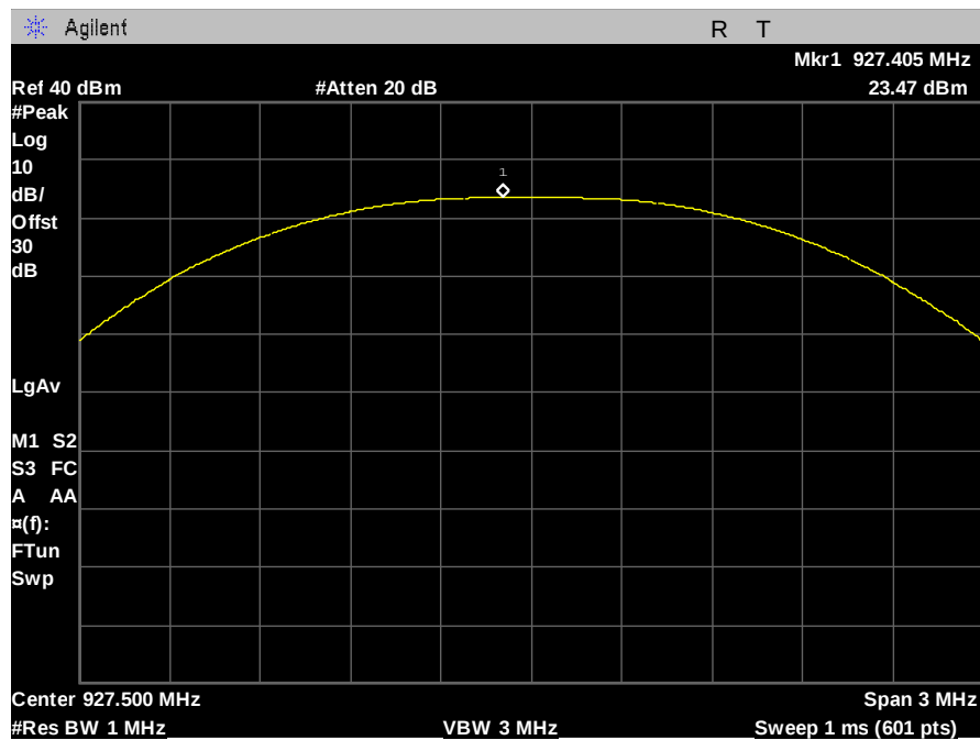
Figure 19: Peak Power - 500kbps - 12dBi - high channel
