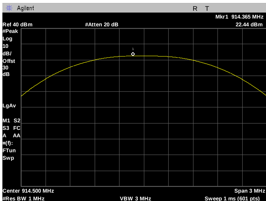
Figure 21: Peak Power - 500kbps - 12dBi - mid channel
