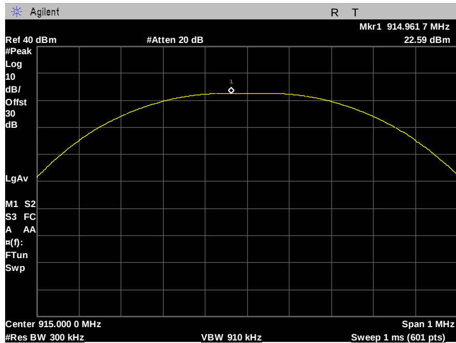
Figure 3: Peak Power - 125kbps - 12dBi - mid channel
