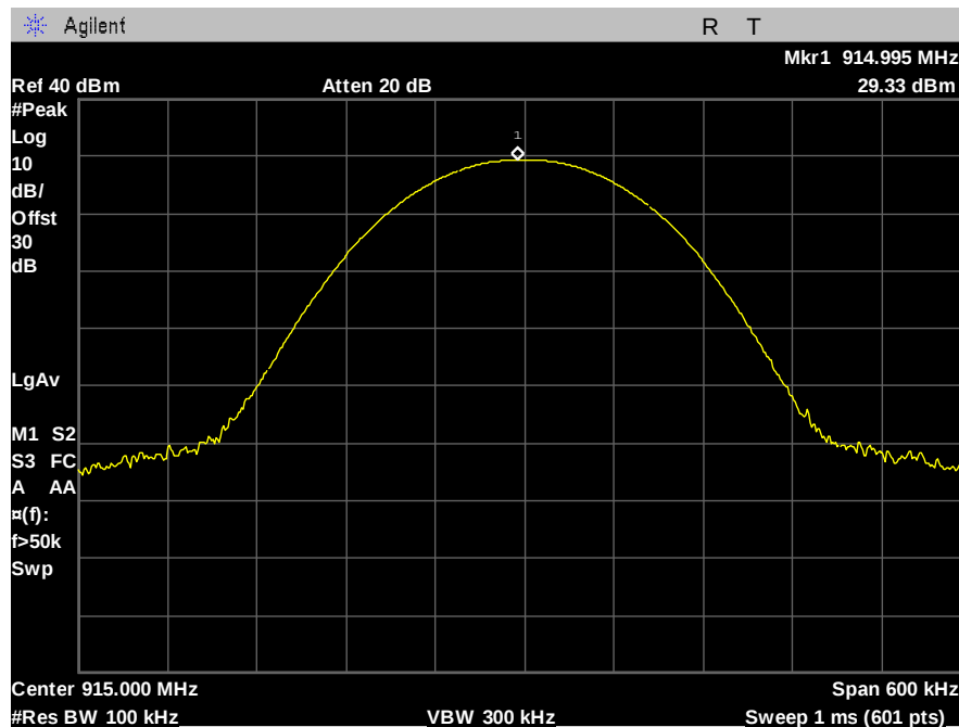
Figure 12: Peak Power - 16kbps - 1dBi - mid channel
