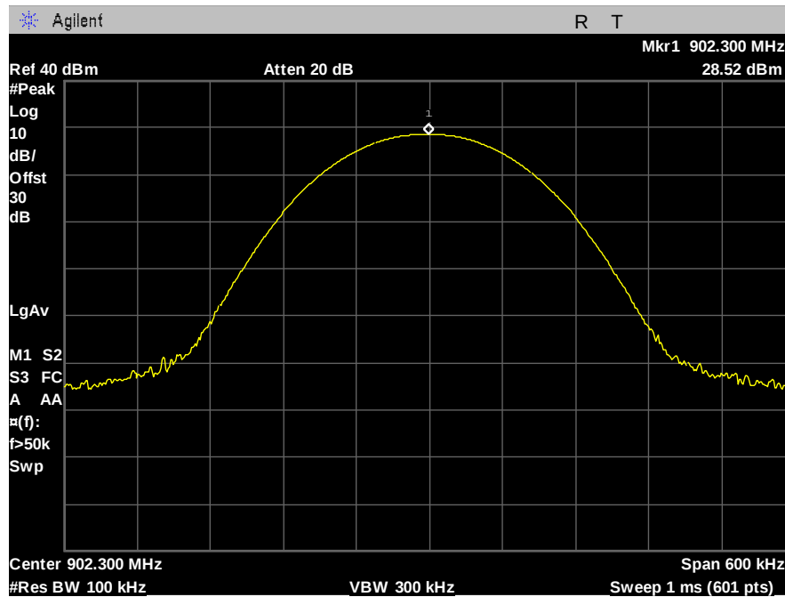
Figure 11: Peak Power - 16kbps - 1dBi - low channel
