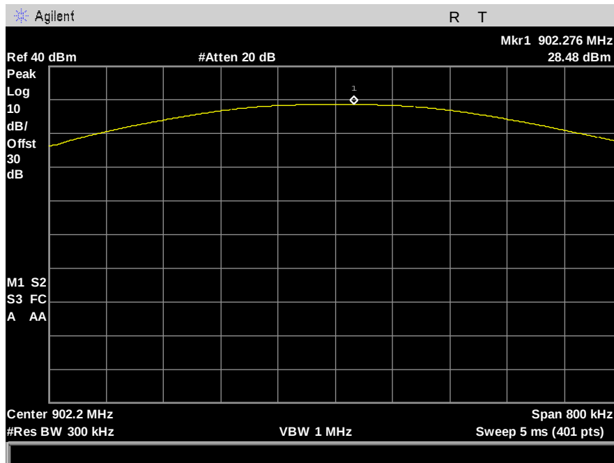
Figure 5: Peak Power - 125kbps - 1dBi - low channel
