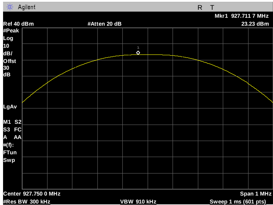
Figure 1: Peak Power - 125kbps - 12dBi - high channel
