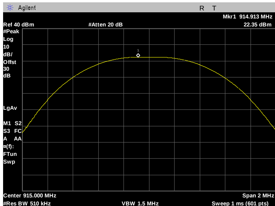
Figure 15: Peak Power - 250kbps - 12dBi - mid channel
