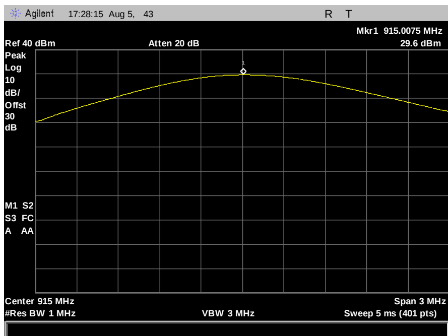
Figure 24: Peak Power - 500kbps - 1dBi - mid channel
