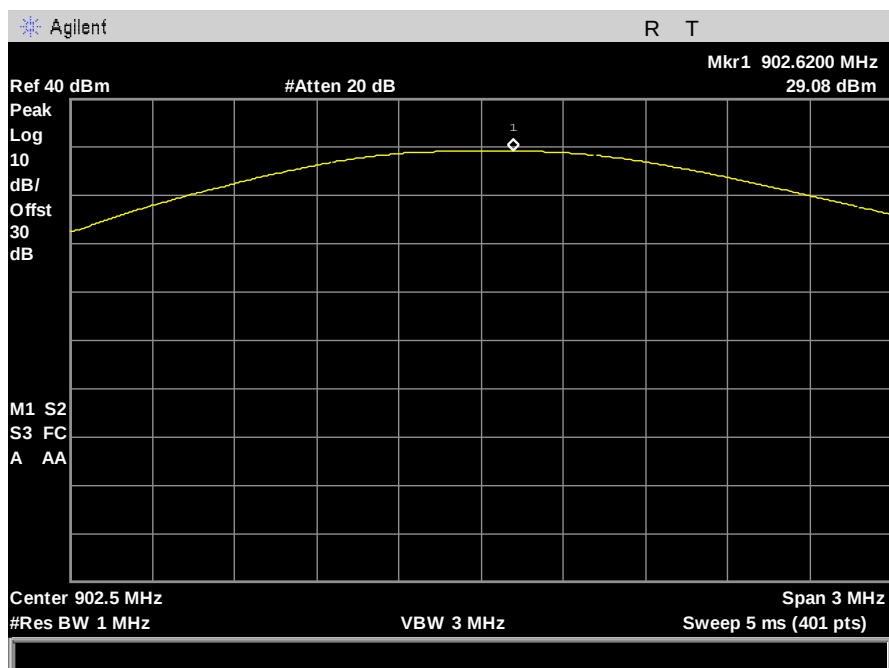
Figure 23: Peak Power - 500kbps - 1dBi - low channel
