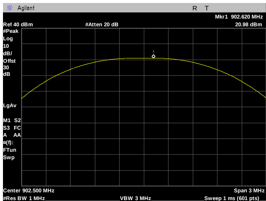
Figure 20: Peak Power - 500kbps - 12dBi - low channel
