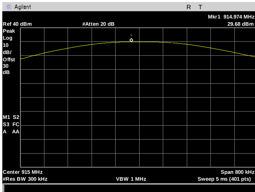
Figure 6: Peak Power - 125kbps - 1dBi - mid channel
