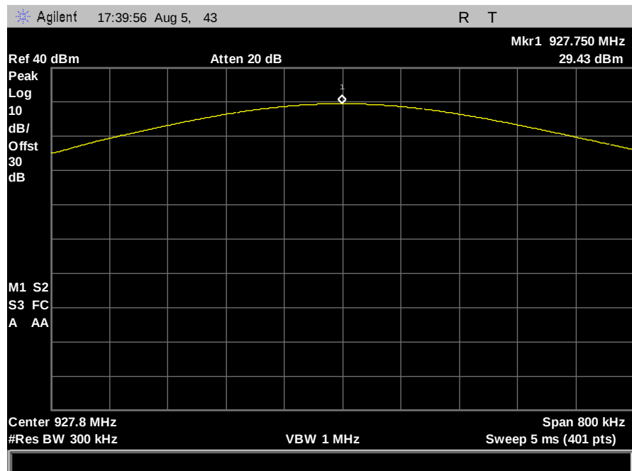
Figure 4: Peak Power - 125kbps - 1dBi - high channel
