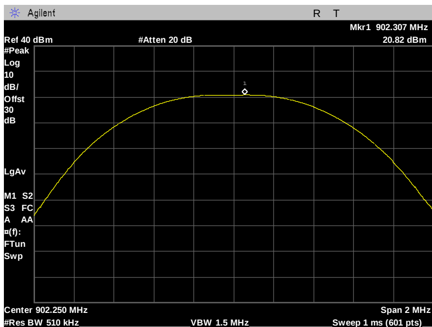
Figure 14: Peak Power - 250kbps - 12dBi - low channel
