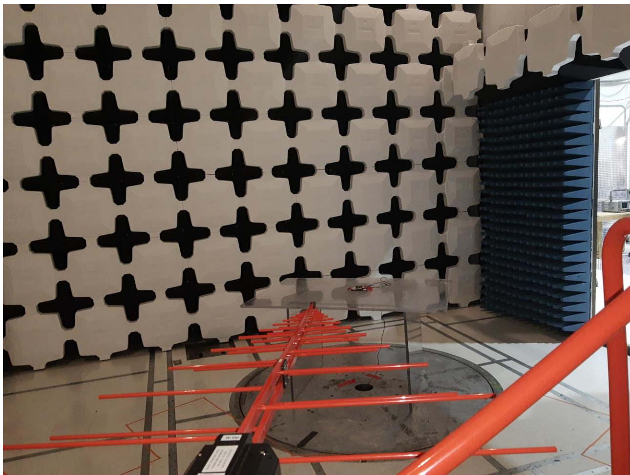
Figure 4: Radiated Emissions Test Setup - 30-1000MHz - 1dBi configuration
