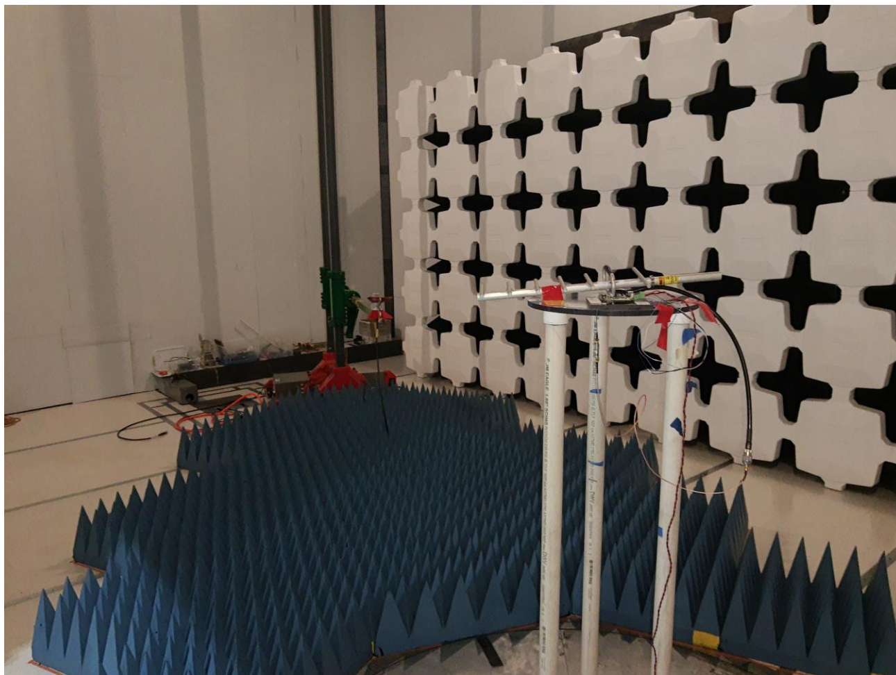
Figure 1: Radiated Emissions Test Setup - 1-10GHz - 12dBi configuration
