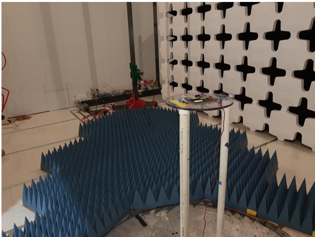
Figure 2: Radiated Emissions Test Setup - 1-10GHz - 1dBi configuration
