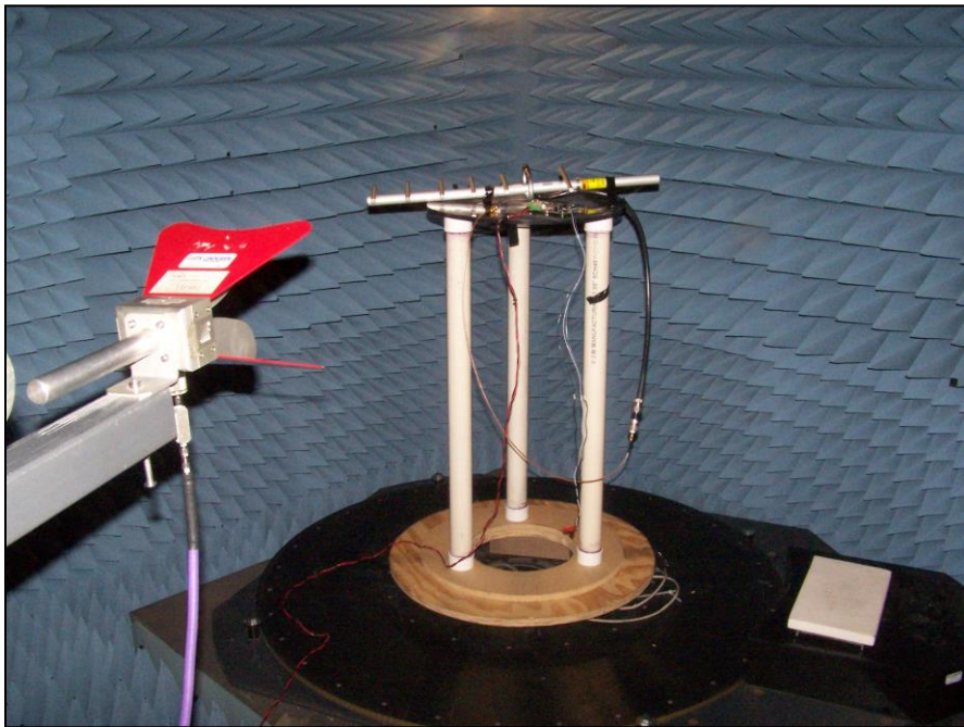
Photograph 9. Radiated Spurious Emissions, Test Setup, Above 1 GHz, 12 dBi Antenna
