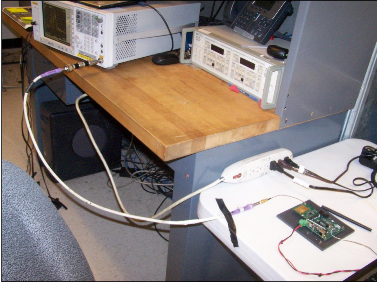
Photograph 4. Channel Separation, Test Setup
