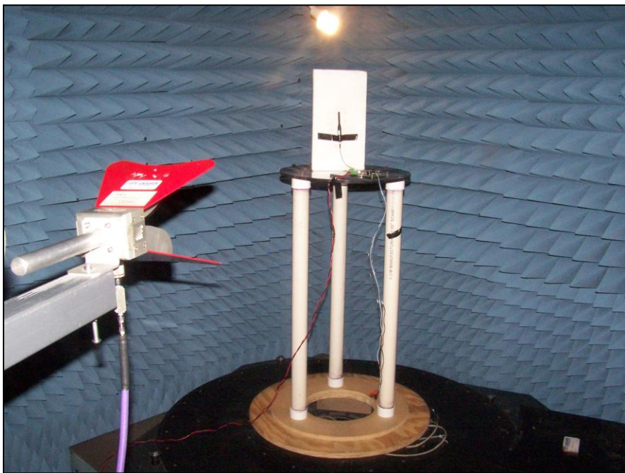
Photograph 7. Radiated Spurious Emissions, Test Setup, Above 1 GHz, 1 dBi Antenna
