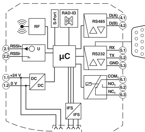
Figure 2 Circuit diagram
