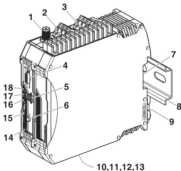
Figure 1 RAD-900-IFS
