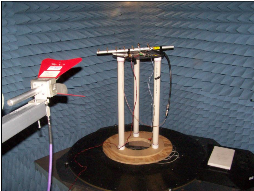
Photograph 6. Radiated Spurious Emissions, Test Setup, Above 1 GHz, 12 dBi Antenna
