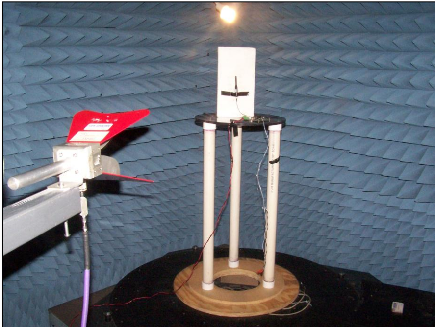
Photograph 4. Radiated Spurious Emissions, Test Setup, Above 1 GHz, 1 dBi Antenna
