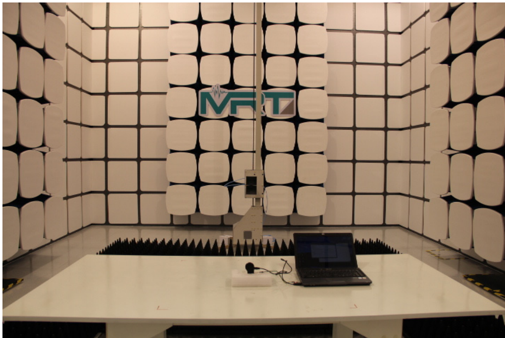
Description: Radiated Emission Test Setup for 1~18GHz
