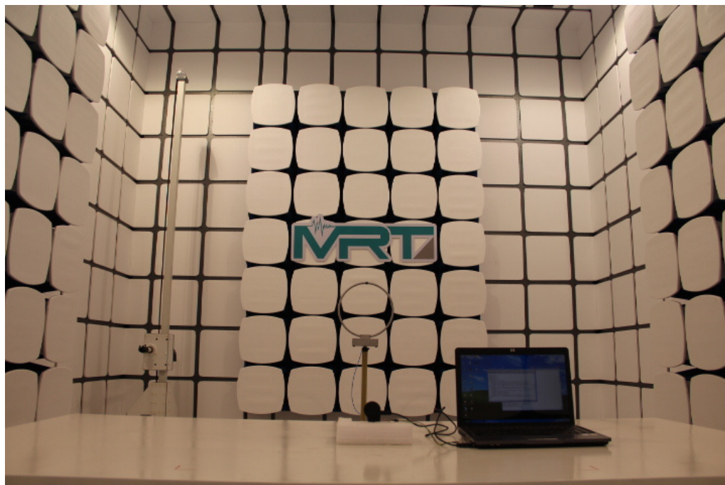
Description: Radiated Emission Test Setup for Below 30MHz
