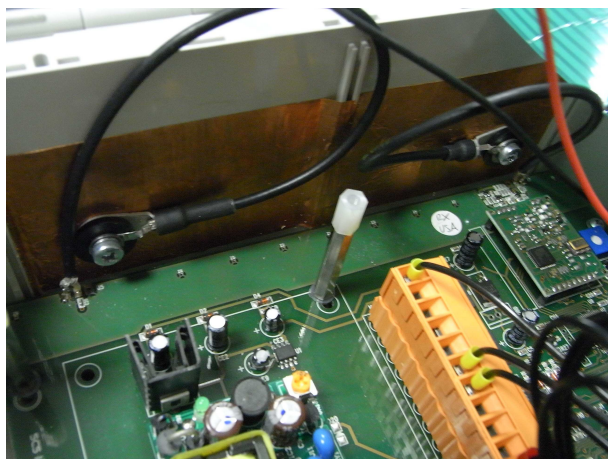
Particular of antenna connection and radio module
