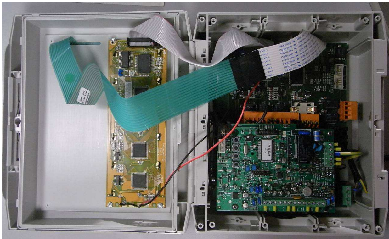
Particular of antenna connection and radio module
