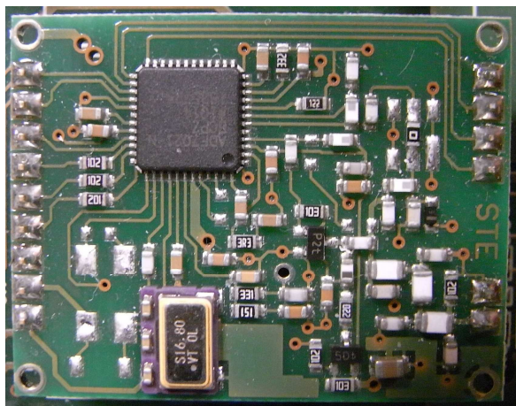
Particular of antenna connection and radio module
