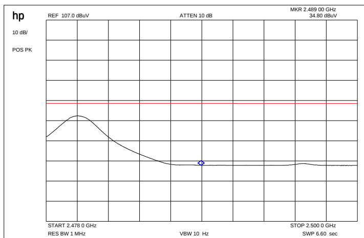
Plot 5: Restricted Bands high
