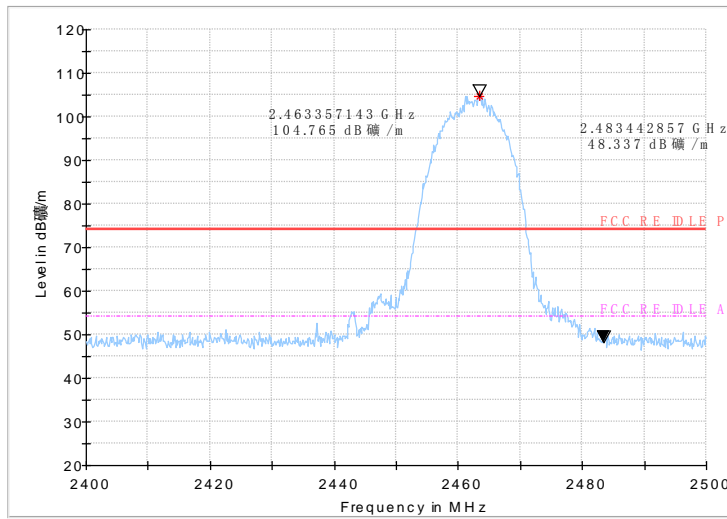
Fig.45 Radiated emission (Power): 802.11b, high channel
