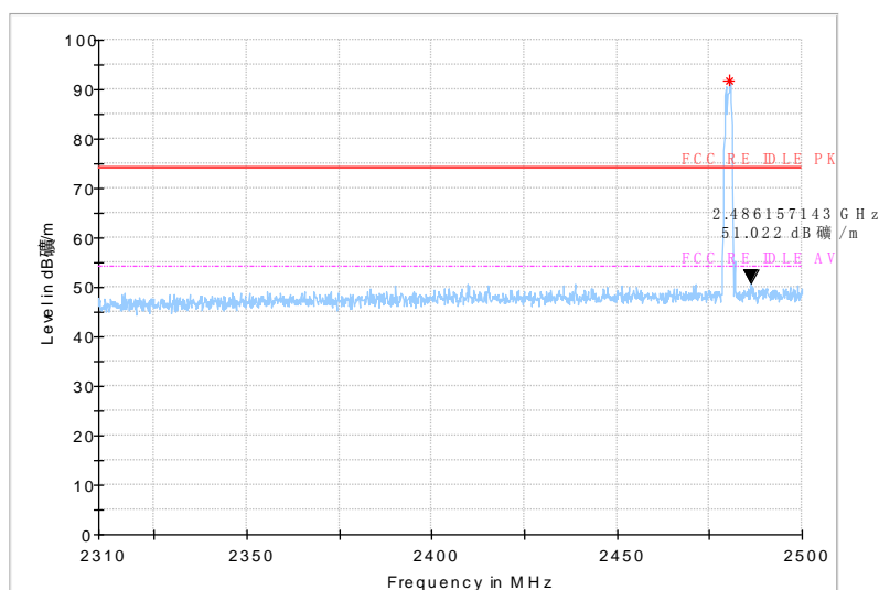
Fig.22 Radiated emission (Power): high channel
