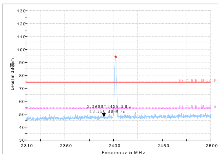
Fig.21 Radiated emission (Power): low channel
