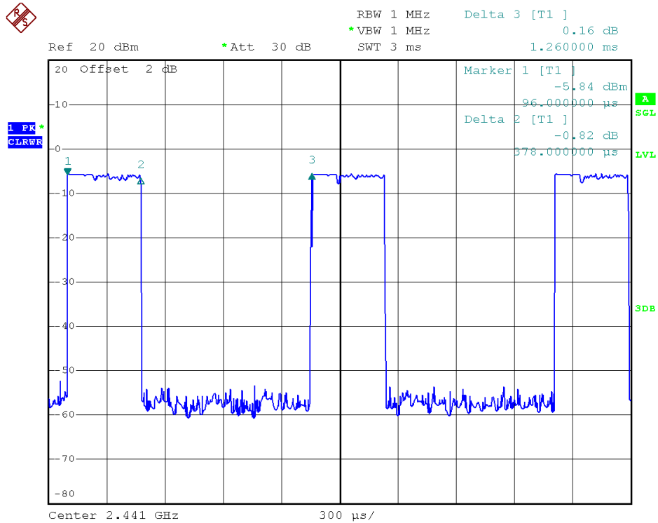
39 Channel @ 3DH1
