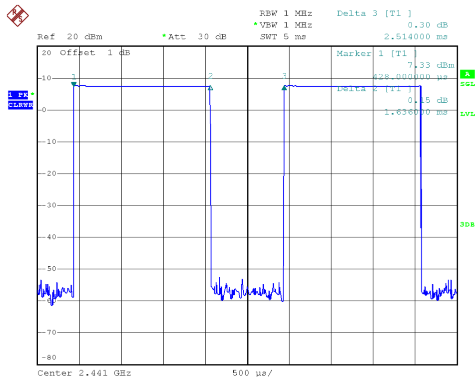
39 Channel @ DH3
