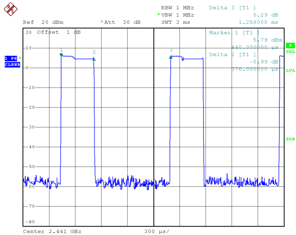
39 Channel @ 2DH1
