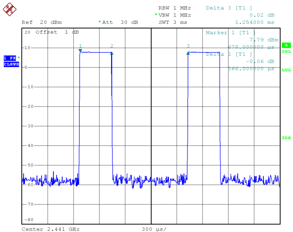
39 Channel @ DH1
