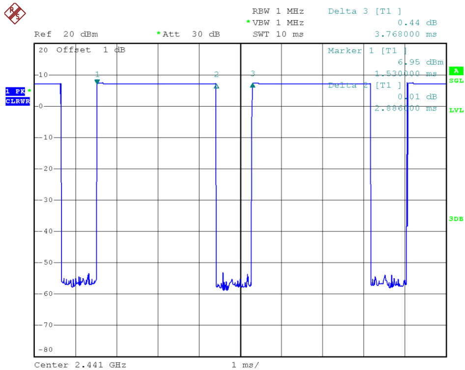
39 Channel @ DH5
