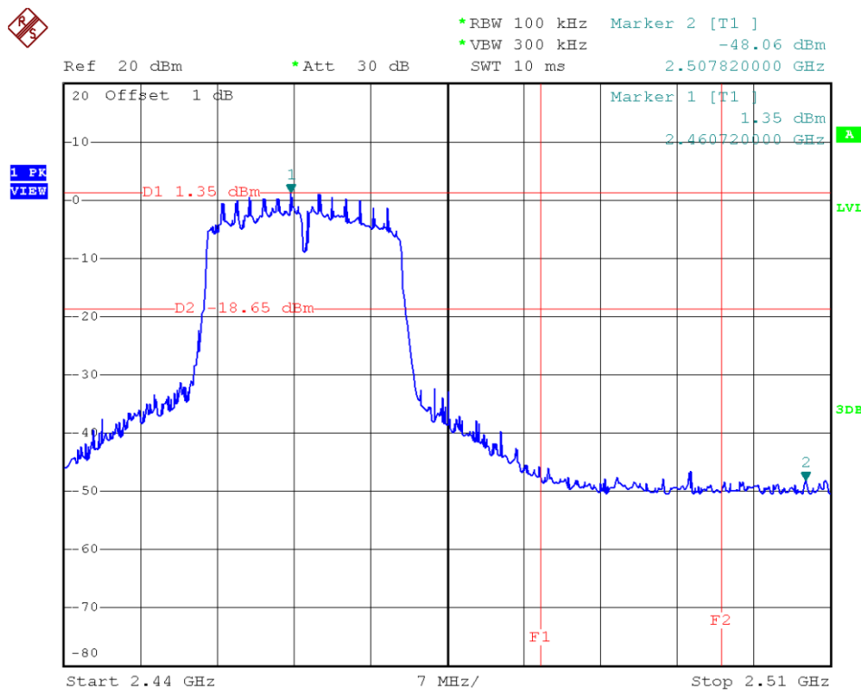
802.11n20 - High Band Edge Plot on Channel 11
