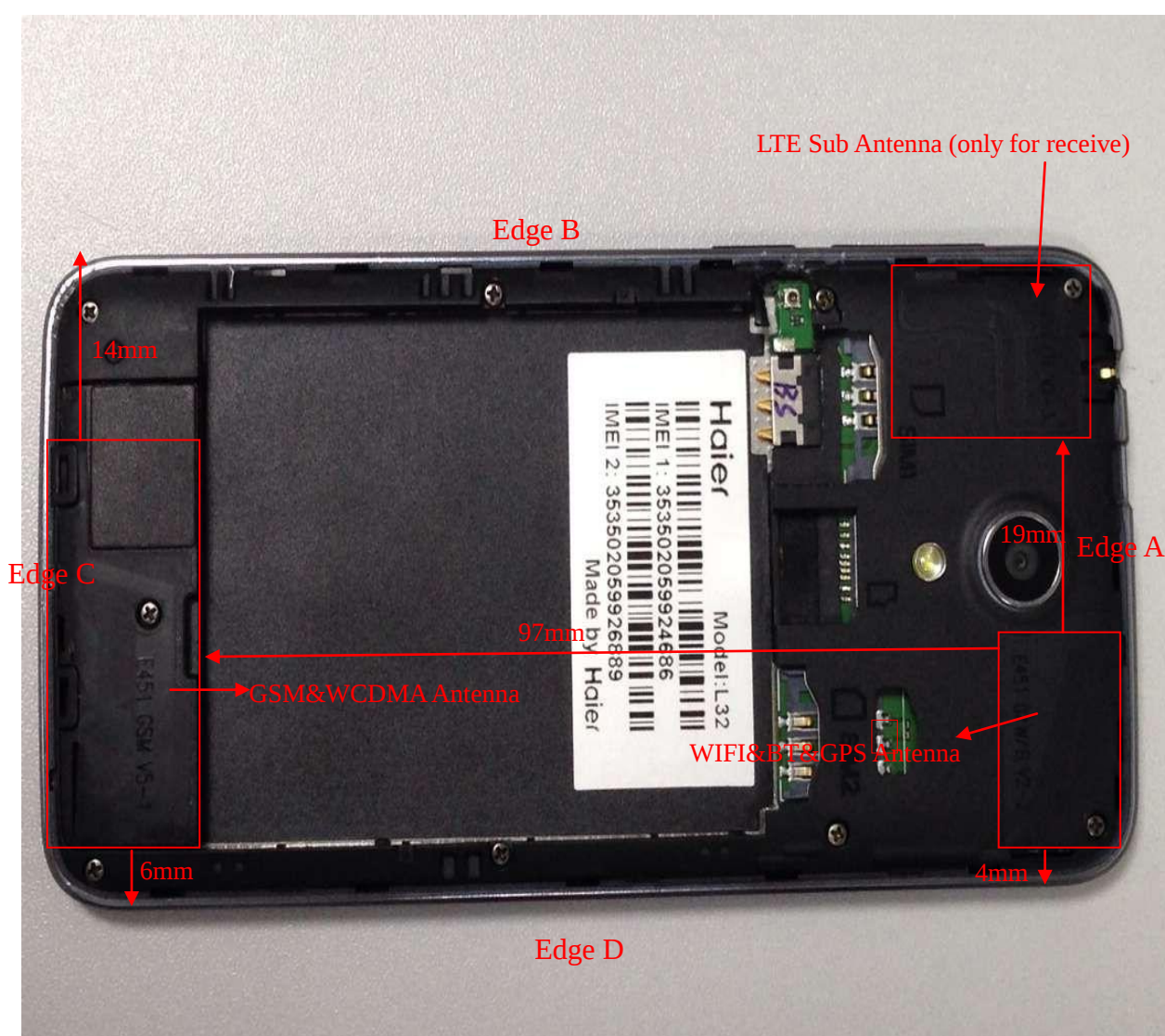
Fig. 3 Position of the antennas
