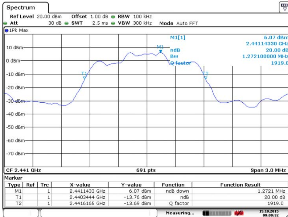
(Plot H: 39 Channel @ 8-DPSK)
