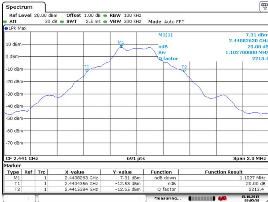
(Plot B: 39 Channel @ GFSK)
