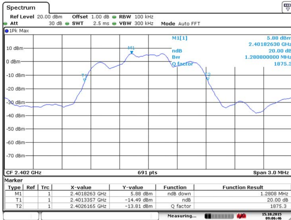
(Plot D: 0 Channel @ \pi/4 -DQPSK)
