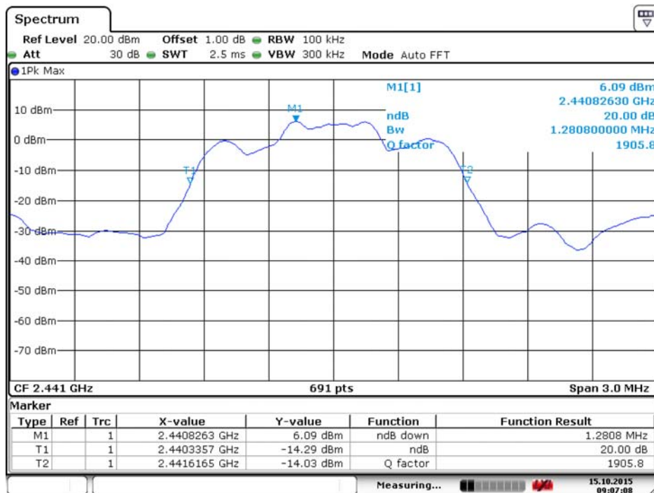
(Plot E: 39 Channel @ \pi/4 -DQPSK)
