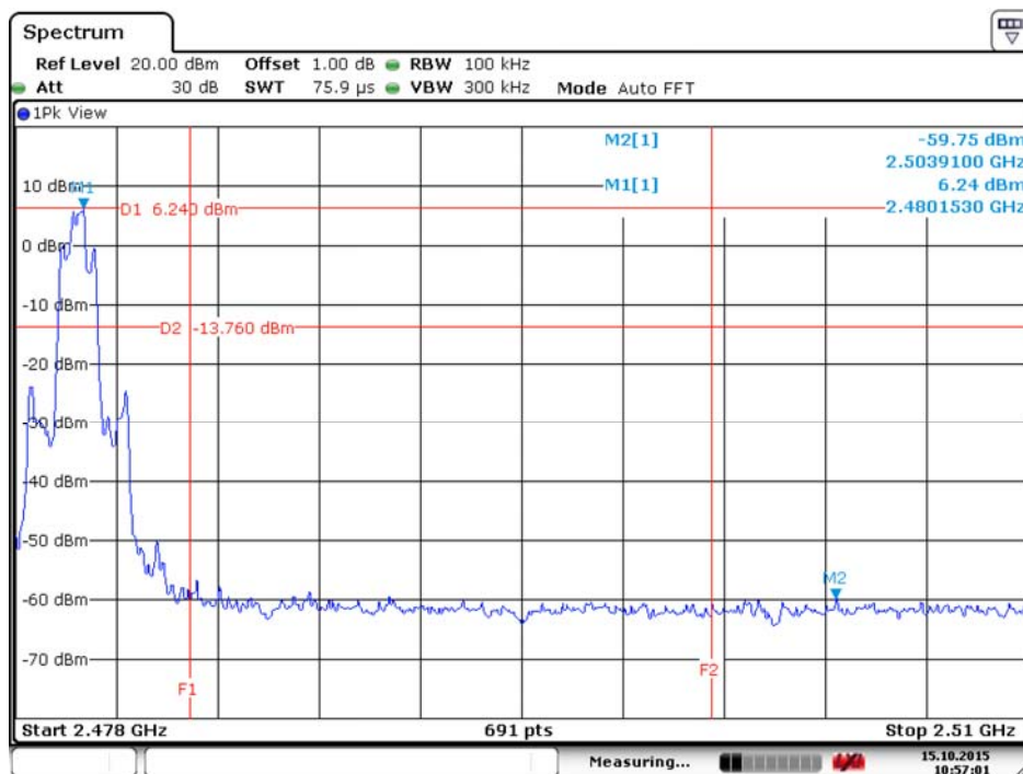
High Band Edge Plot on channel 78 @8-DPSK
