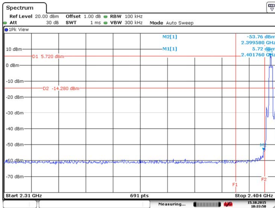
Low Band Edge Plot on channel 0 @8-DPSK
