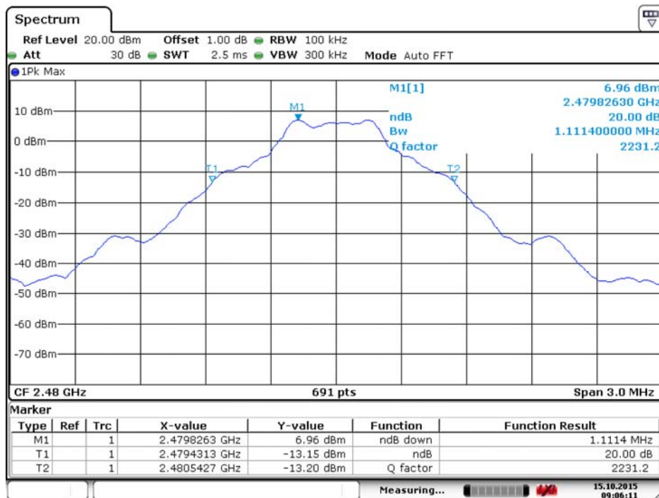
(Plot C: 78 Channel @ GFSK)
