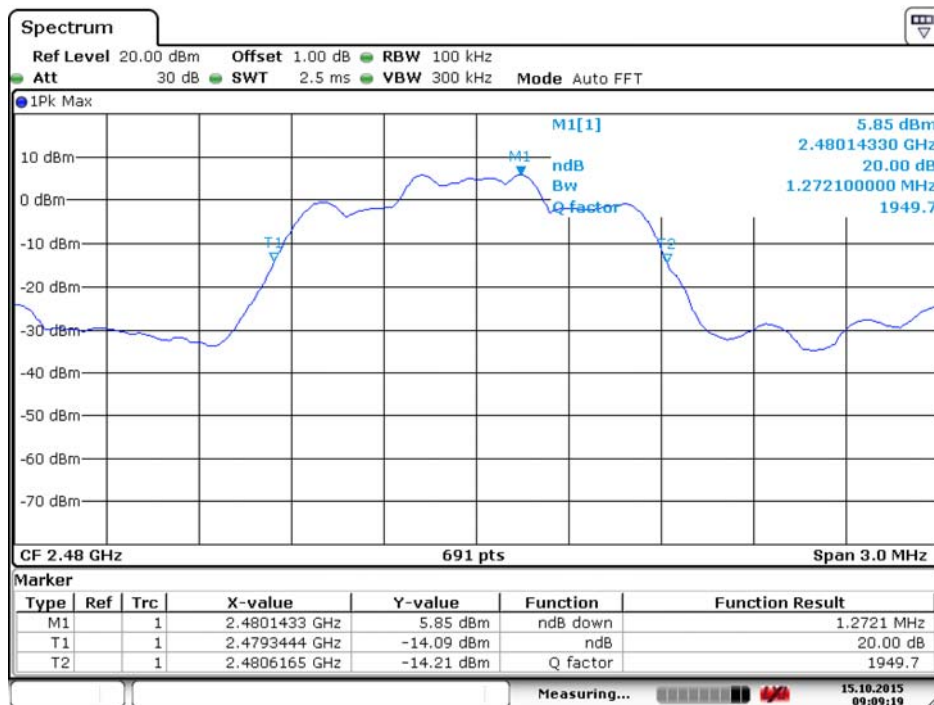
(Plot I: 78 Channel @ 8-DPSK)
