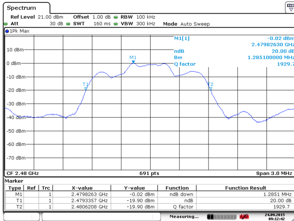
(Plot F: 78 Channel @ \pi/4 -DQPSK)
