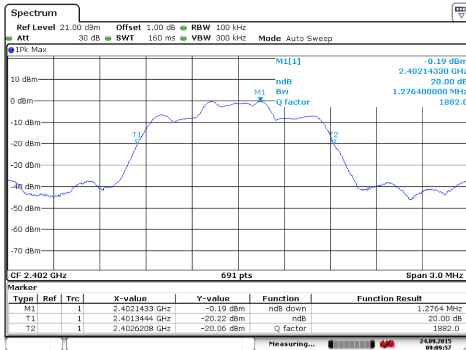
(Plot G: 0 Channel @ 8-DPSK)
