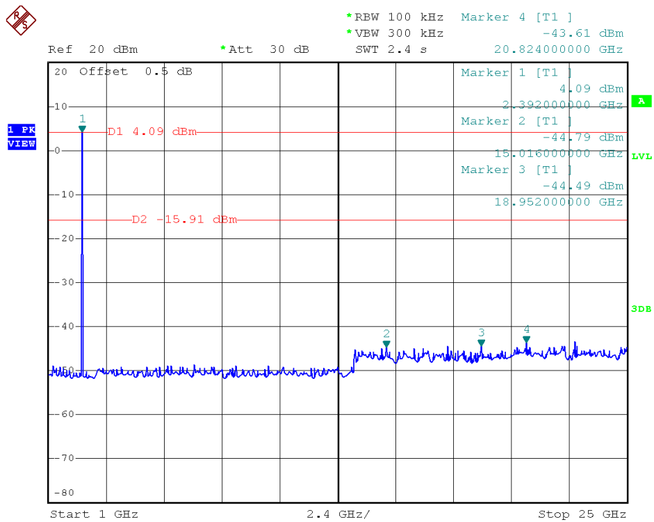
Channel = 0, 1GHz to 25GHz @ \pi/4 -DQPSK
