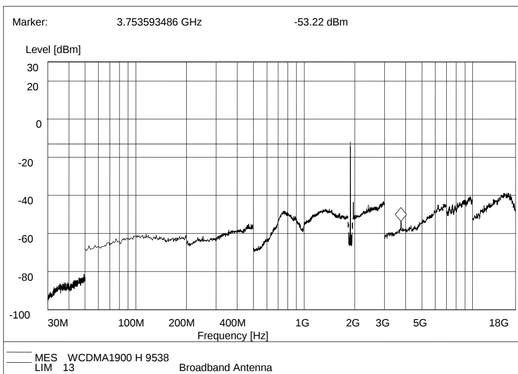
(Plot D.5: WCDMA 1900MHz Channel = 9538, Test Antenna Horizontal)
