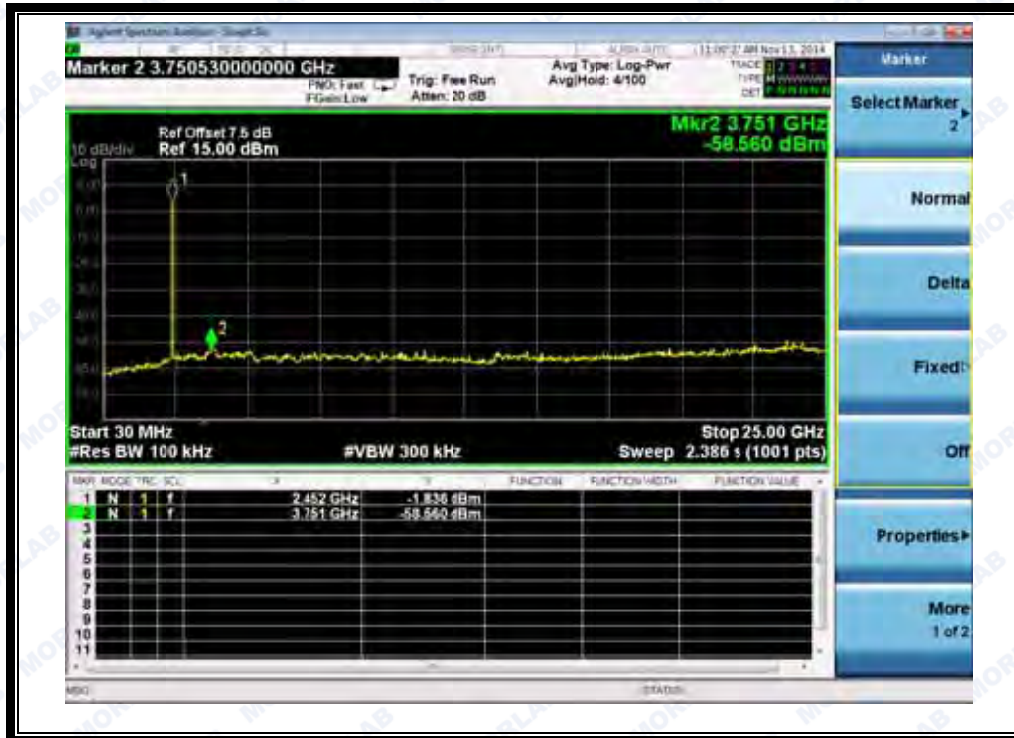
(Plot H.1: Channel = 39, 30MHz to 25GHz @ 8-DPSK)
