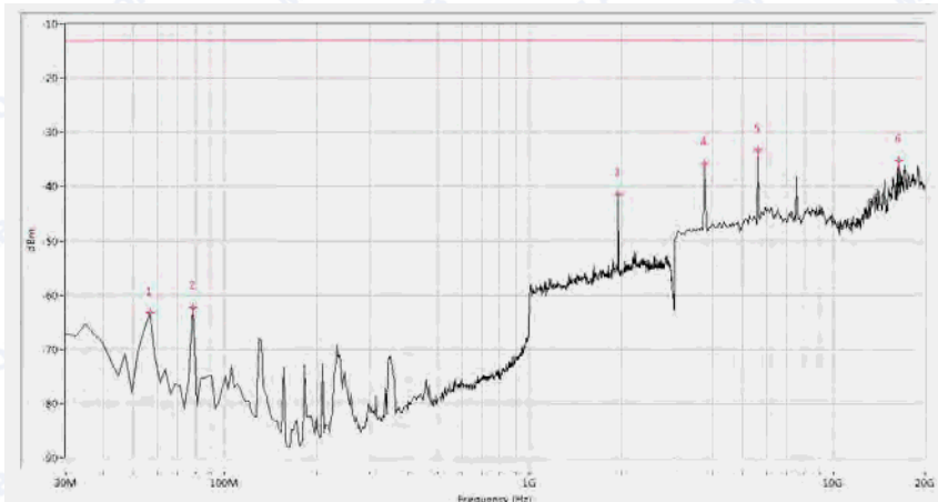
(Plot B.4: GSM 1900MHz Channel = 661, Test Antenna Vertical)
