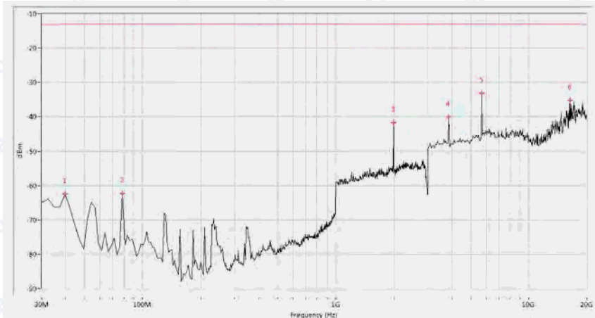
(PlotB.6: GSM 1900MHz Channel = 810, Test Antenna Vertical)
