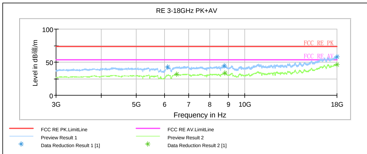
Radiated Emission from 3GHz to 18GHz
