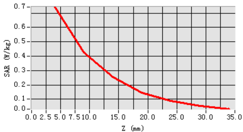
SAR, Z Axis Scan (X = -13, Y = -20)
