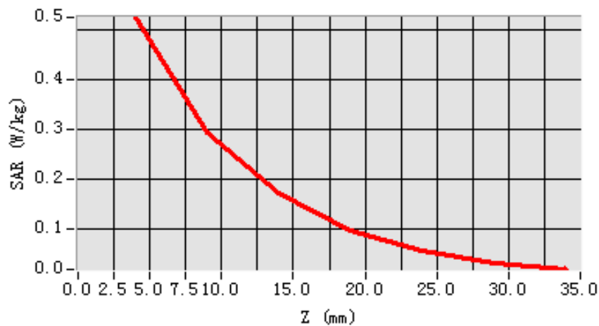
SAR, Z Axis Scan (X = -11, Y = -18)
