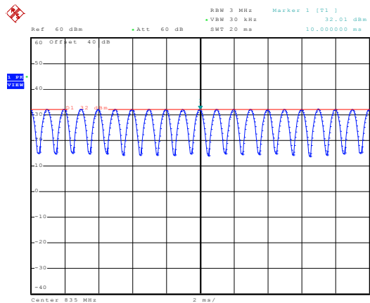
835MHz - 80% AM
