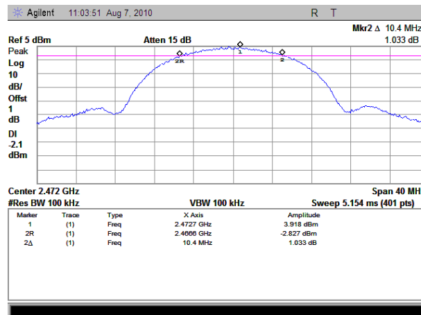
(Plot C: Channel 13: 2472MHz)
