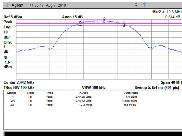
(Plot B: Channel 7: 2442 MHz)
