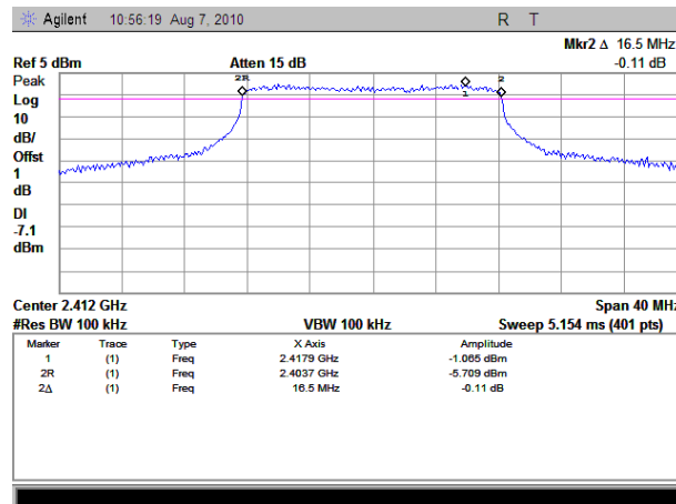
(Plot D: Channel 1: 2412MHz)
