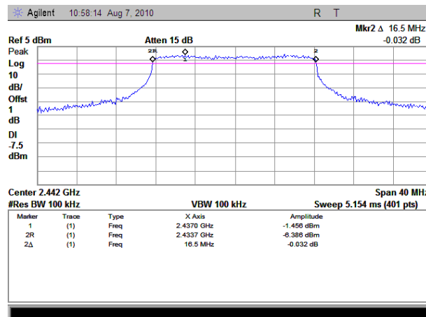
(Plot E: Channel 7: 2442MHz)
