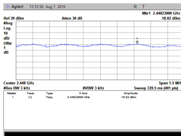
(Plot E: Channel = 7)
