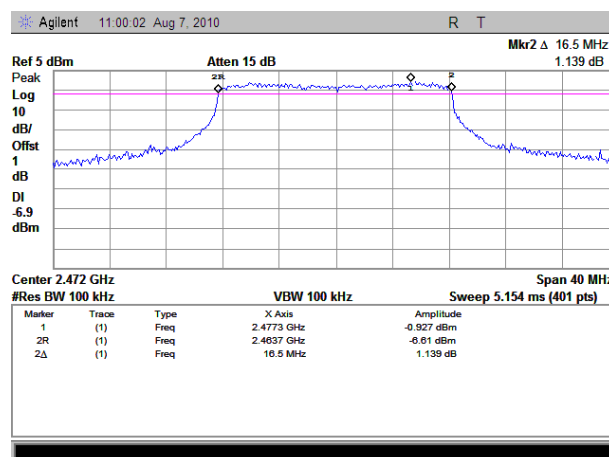
(Plot F: Channel 13: 2472MHz)
