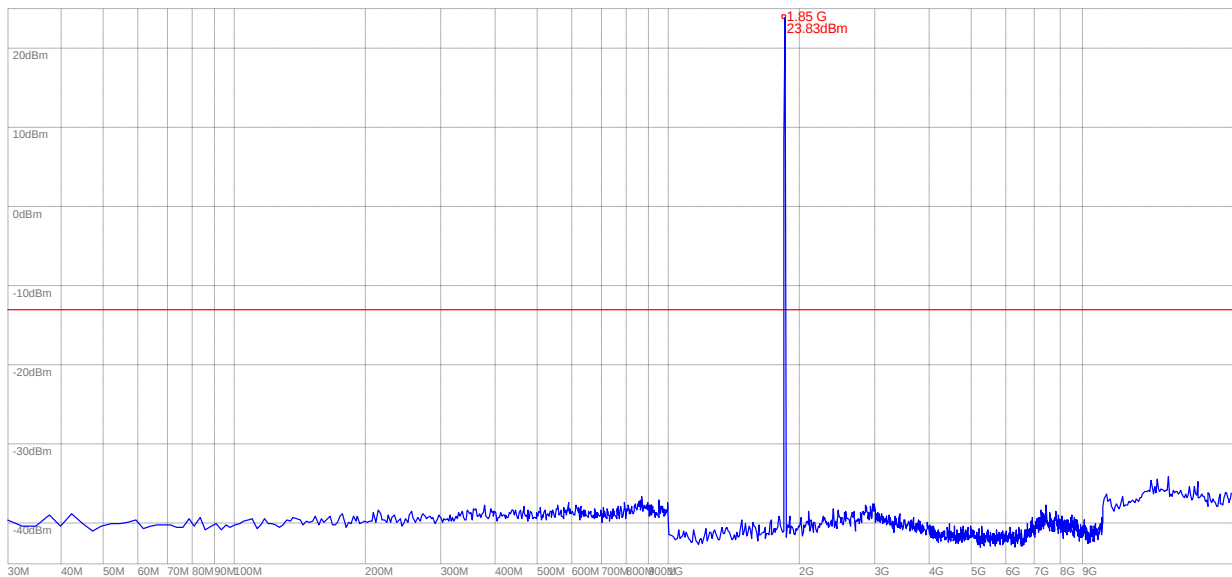
(Plot J: CDMA 1900-EVDO Channel = 25, 30MHz to 20GHz)
