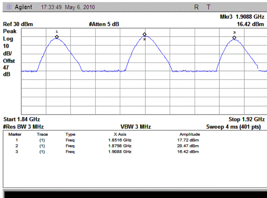
(Plot D: CDMA 1900-EVDO Channel = 25, 600, 1175)
