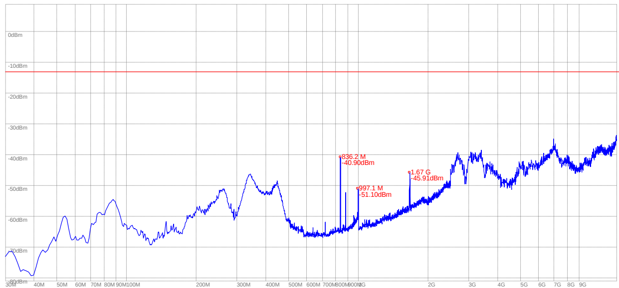
(Plot H.1: CDMA 800-EVDO Channel = 384, Test Antenna Horizontal)
