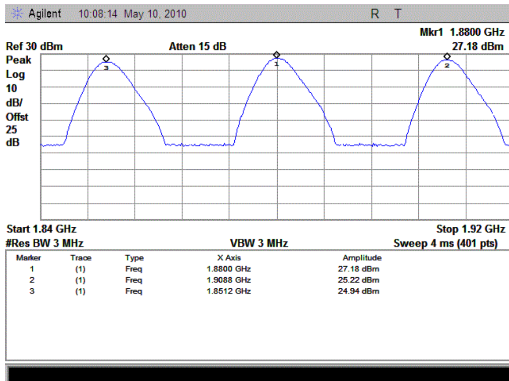
(Plot D: CDMA 1900-EVDO Channel = 25, 600, 1175)
