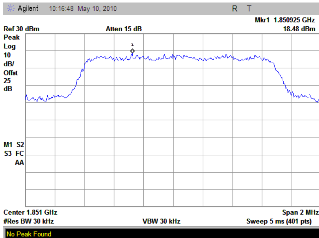
(Plot G: CDMA 1900-EVDO Channel = 25)
