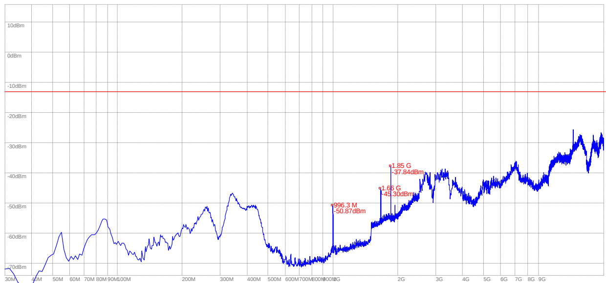
(Plot J.1: CDMA 1900-EVDO Channel = 25, Test Antenna Horizontal)
