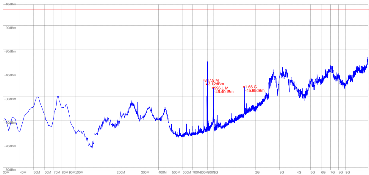
(Plot I.2: CDMA 800-EVDO Channel = 777, Test Antenna Vertical)
