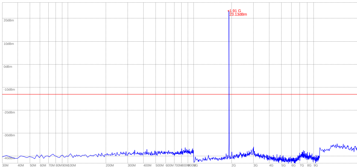
(Plot L: CDMA 1900-EVDO Channel = 1175, 30MHz to 20GHz)
