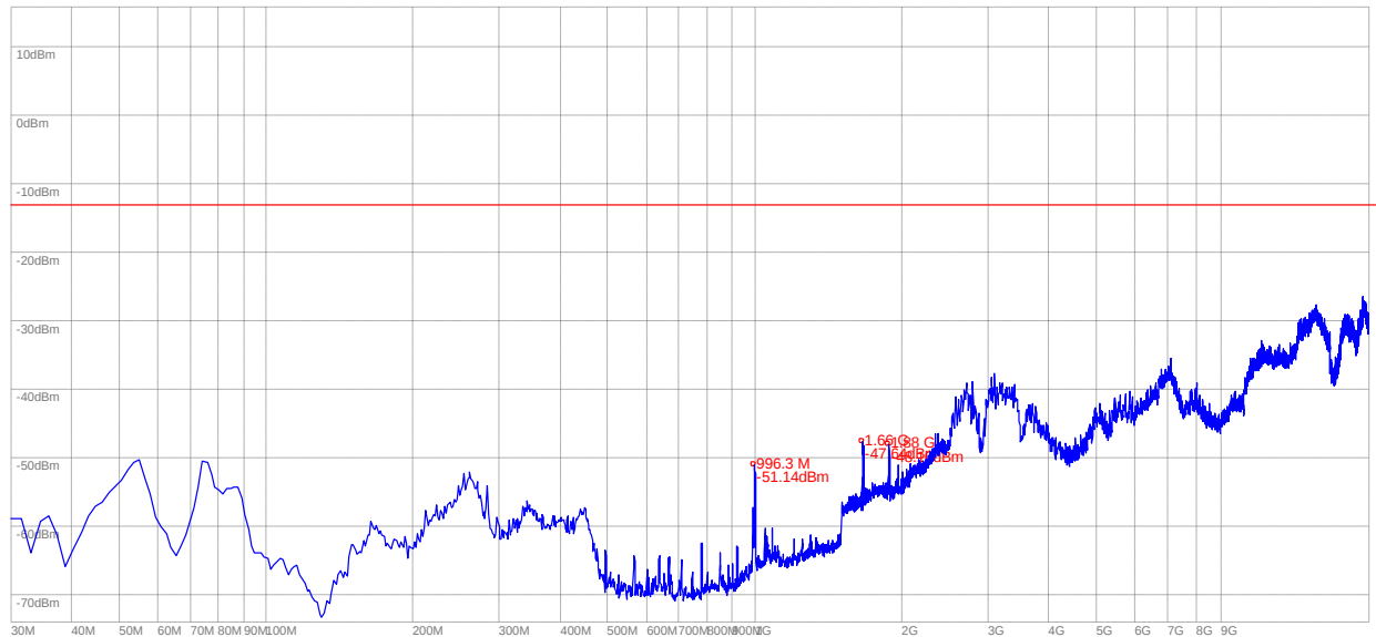
(Plot K.2: CDMA 1900-EVDO Channel = 600, Test Antenna Vertical)
