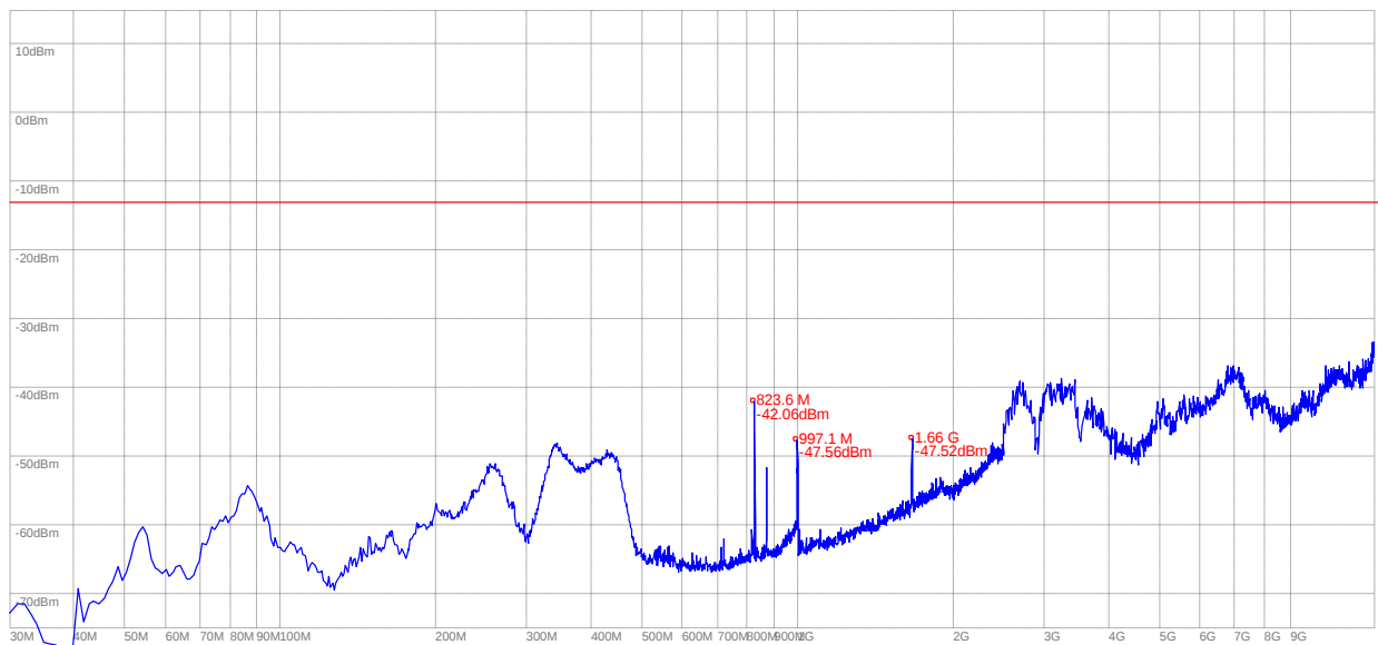
(Plot G.1: CDMA 800-EVDO Channel = 1013, Test Antenna Horizontal)
