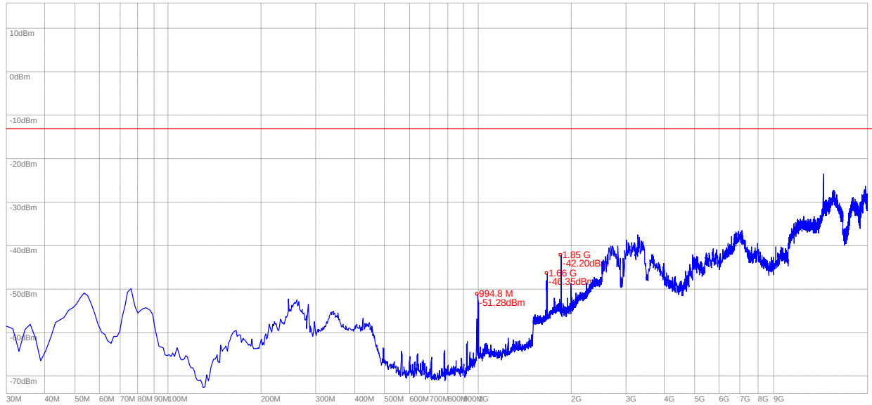
(Plot J.2: CDMA 1900-EVDO Channel = 25, Test Antenna Vertical)
