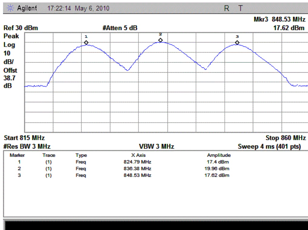
(Plot C: CDMA 800-EVDO Channel = 1013, 384, 777)
