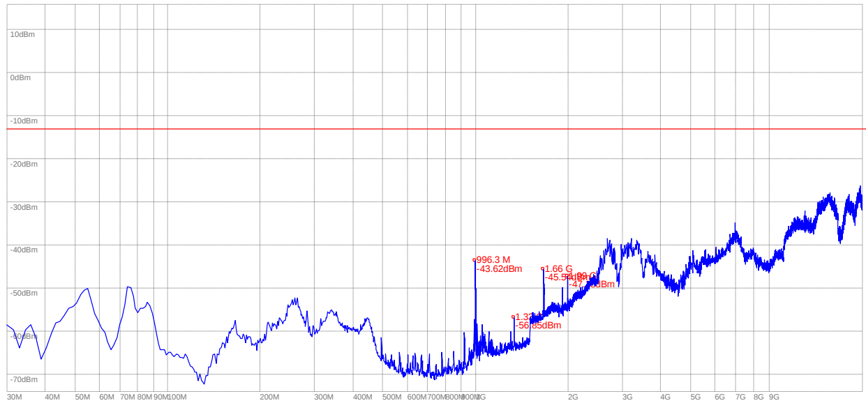
(Plot L.2: CDMA 1900-EVDO Channel = 1175, Test Antenna Vertical)
