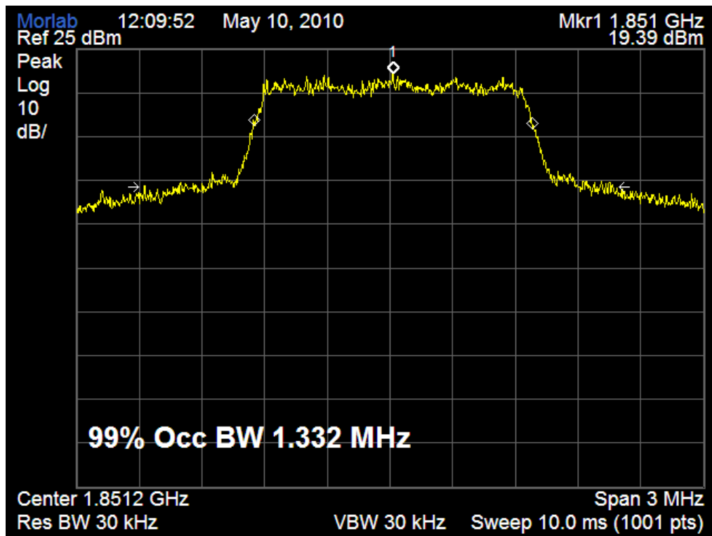
(Plot J: CDMA 1900-EVDO Channel = 25)
