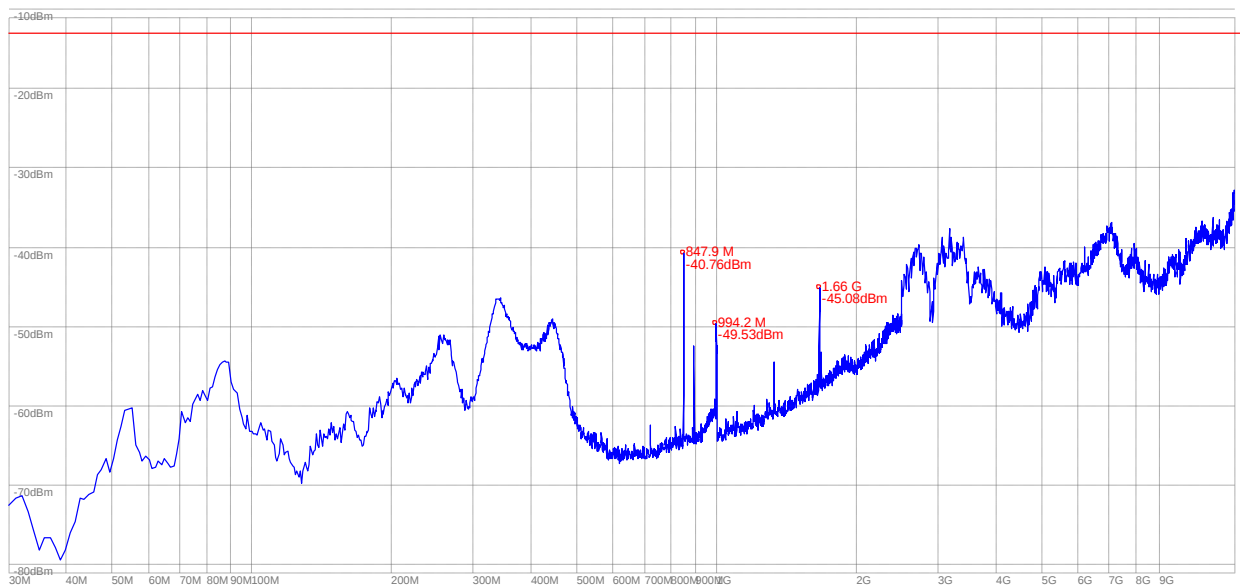
(Plot I.1: CDMA 800-EVDO Channel = 777, Test Antenna Horizontal)
