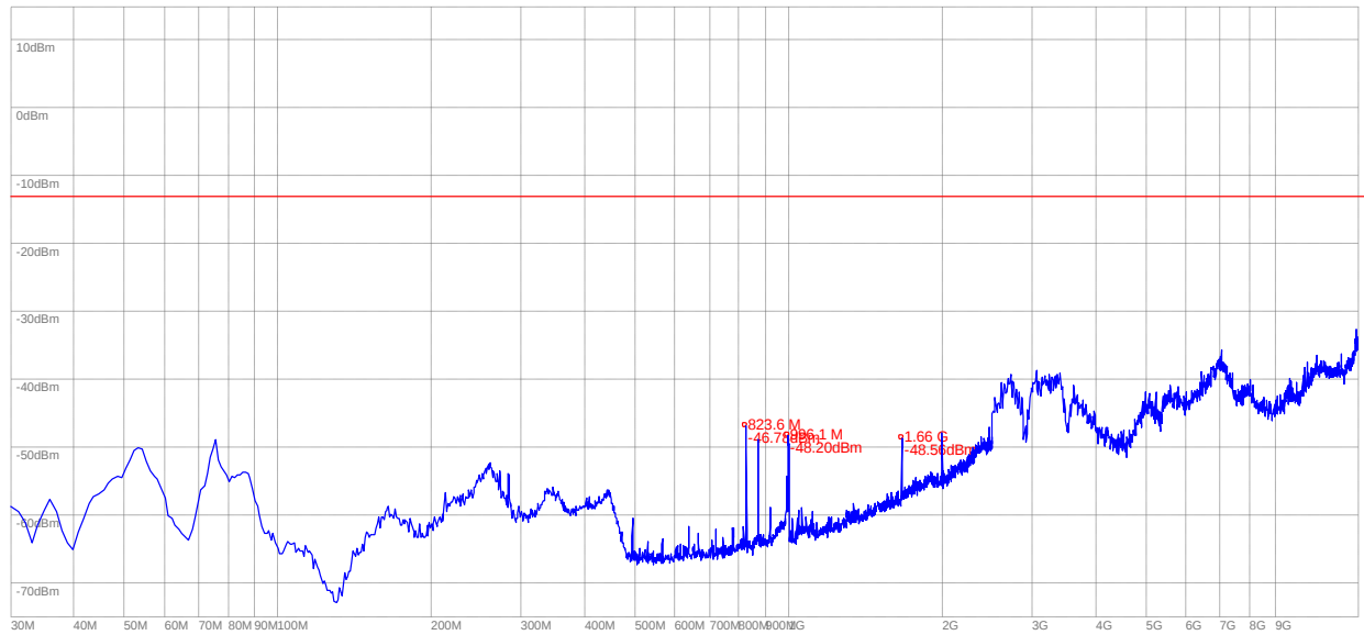
(Plot G.2: CDMA 800-EVDO Channel = 1013, Test Antenna Vertical)
