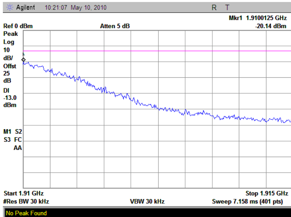
(Plot H: CDMA 1900-EVDO Channel = 1175)
