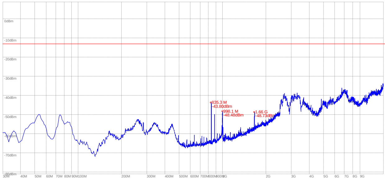
(Plot H.2: CDMA 800-EVDO Channel = 384, Test Antenna Vertical)
