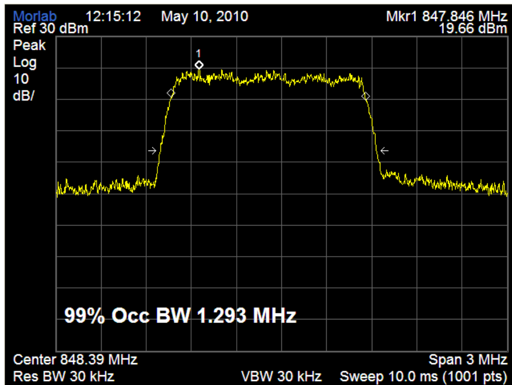
(Plot I: CDMA 800-EVDO Channel = 777)
