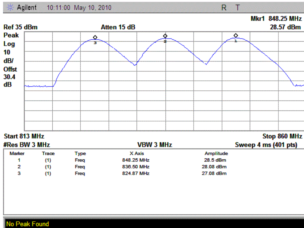
(Plot C: CDMA 800-EBDO Channel = 9, 384, 777)
