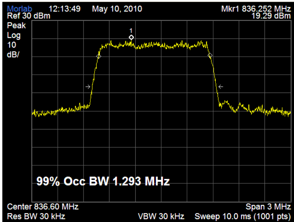
(Plot H: CDMA 800-EVDO Channel = 384)
