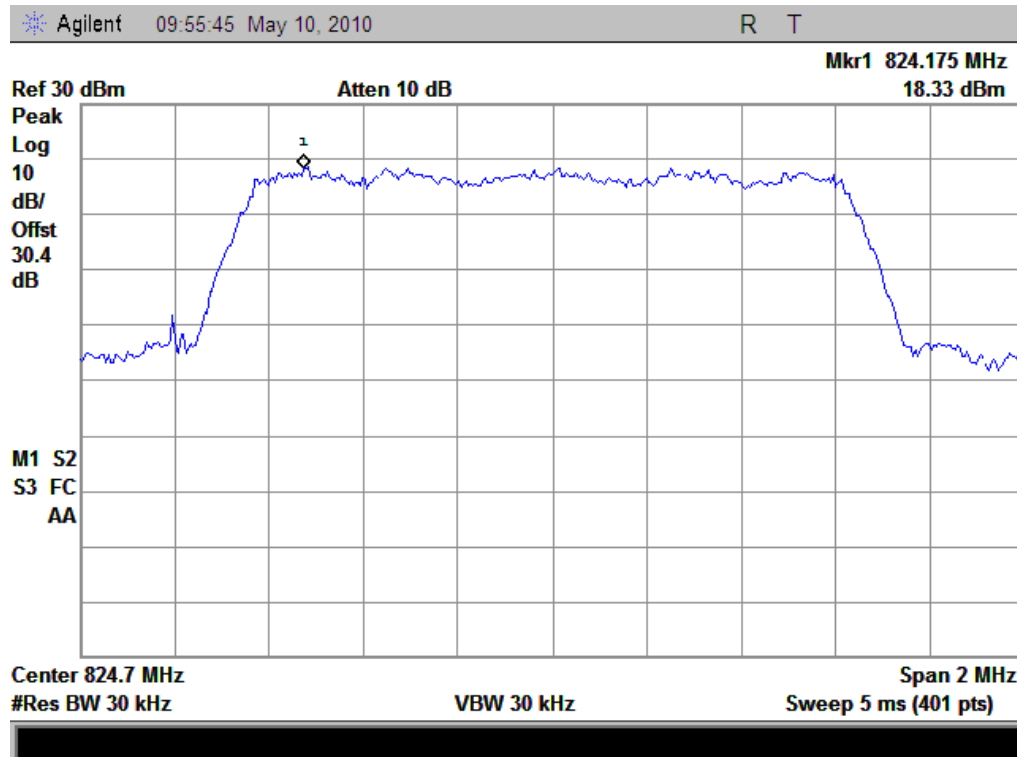
(Plot E: CDMA 800-EVDO Channel = 1013)
