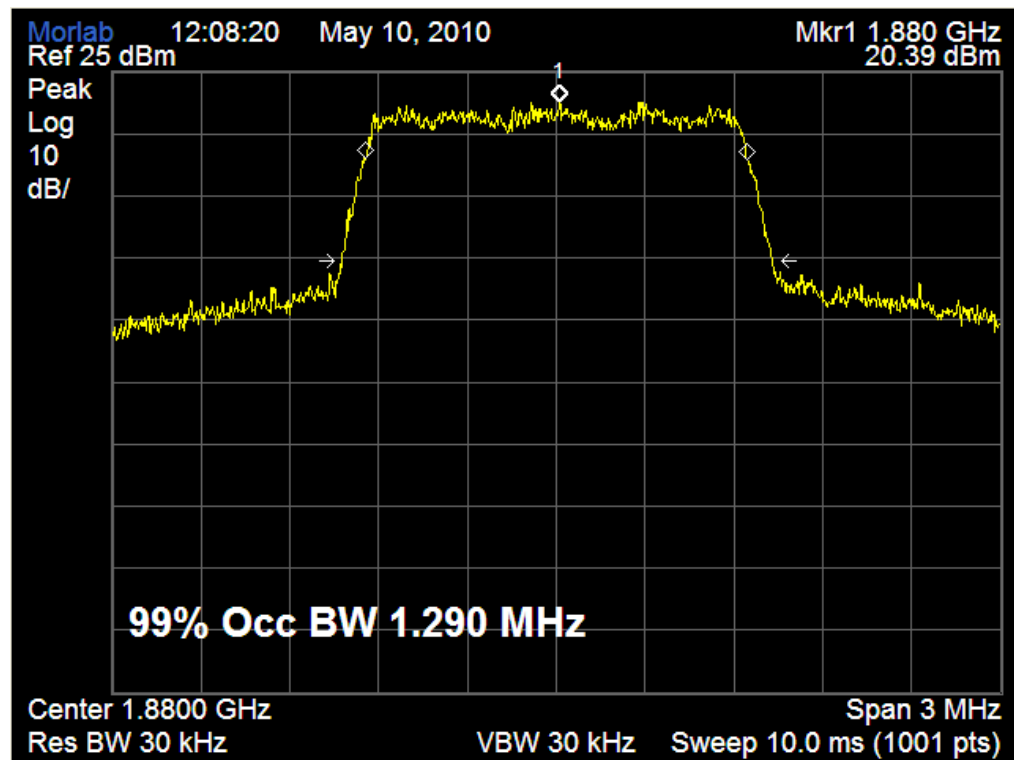
(Plot K: CDMA 1900-EVDO Channel = 600)
