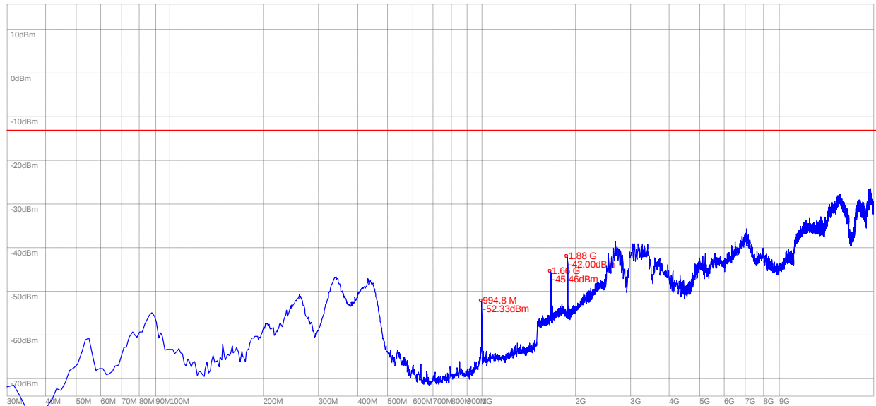
(Plot K.1: CDMA 1900-EVDO Channel = 600, Test Antenna Horizontal)
