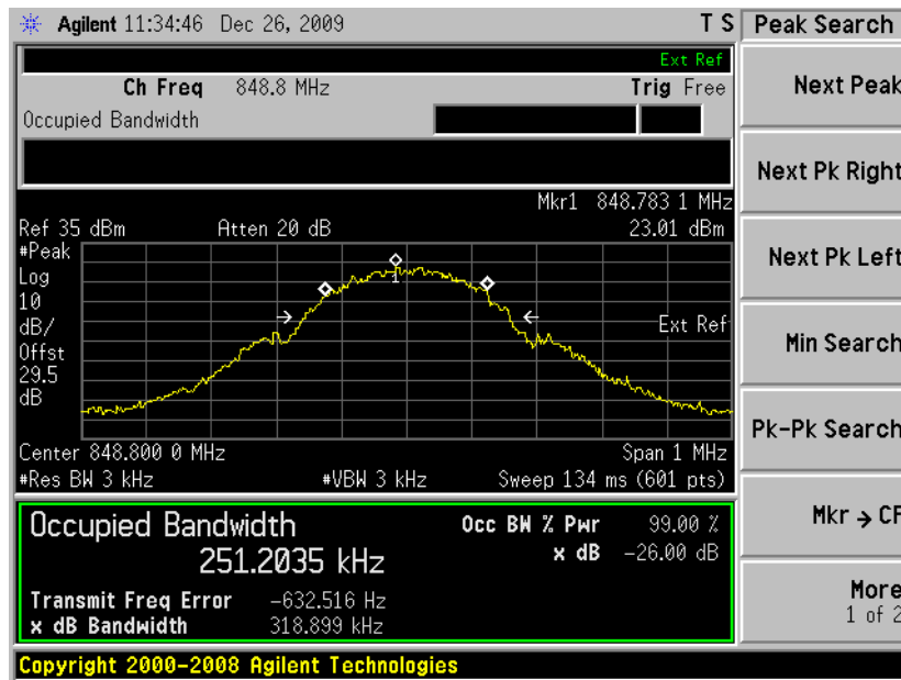
(Plot C: GSM 850MHz Channel = 251)
